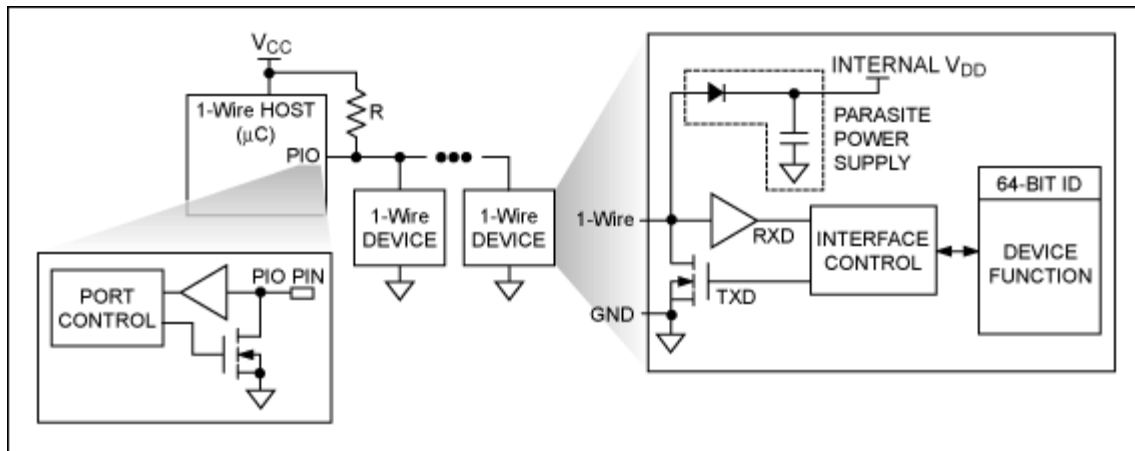
Figure 1. In a 1-Wire master/slave configuration, all devices share a common data line.
