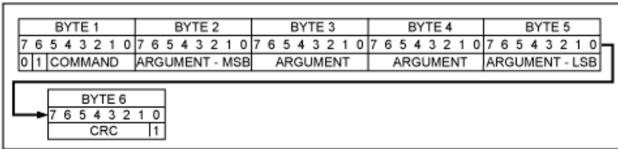
Figure 3. SPI-mode SD commands are issued to the card in a 6-byte format.
