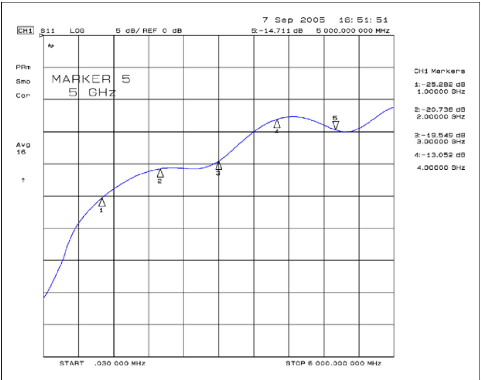
Figure 3. Return loss (S11) of the sealed microcoaxial cable.
