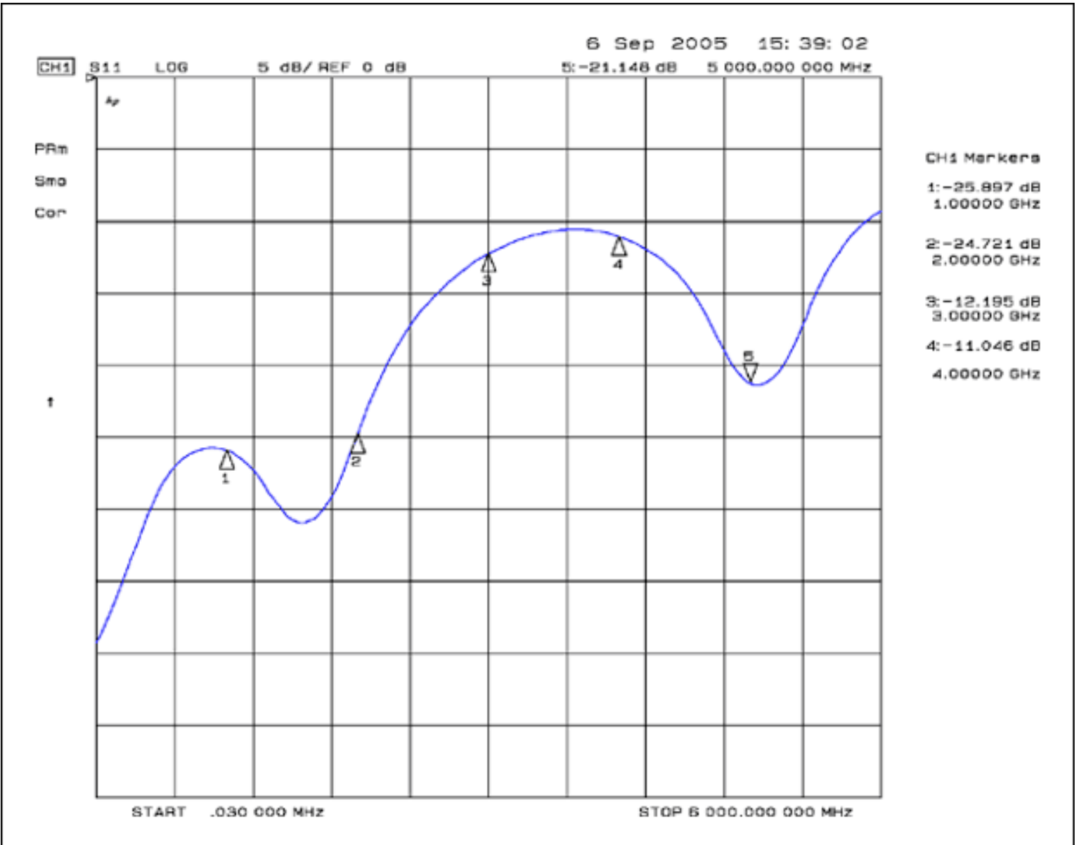
Figure 2b. Return loss (S11) of the handmade microcoaxial cable (terminated to 50Ω on a PCB).
