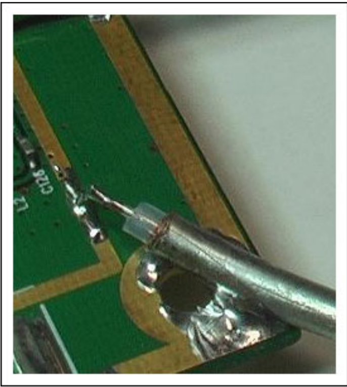
Figure 4a. Excess center conductor length can be detrimental.
