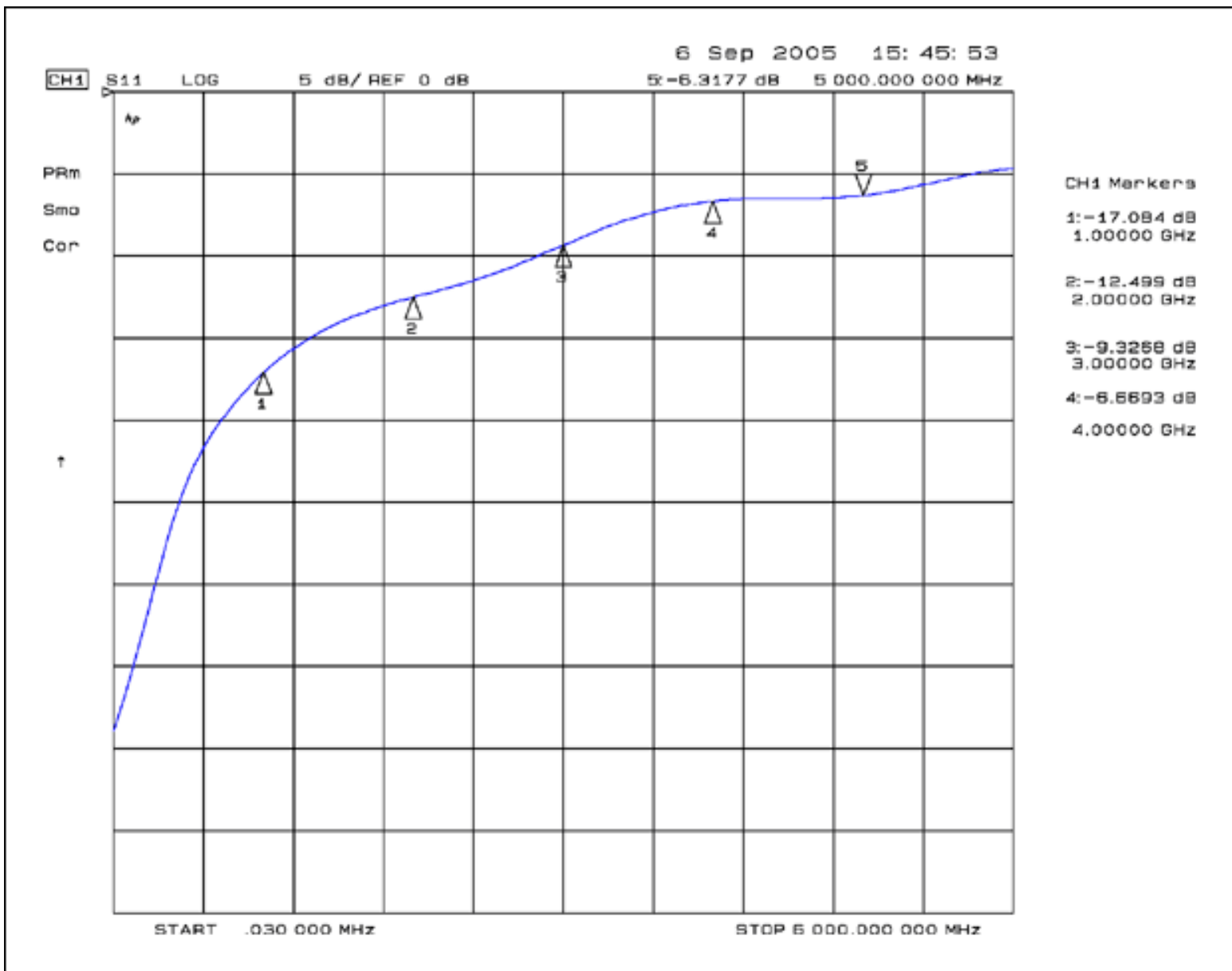
Figure 4b. Return loss with excess center conductor length.
