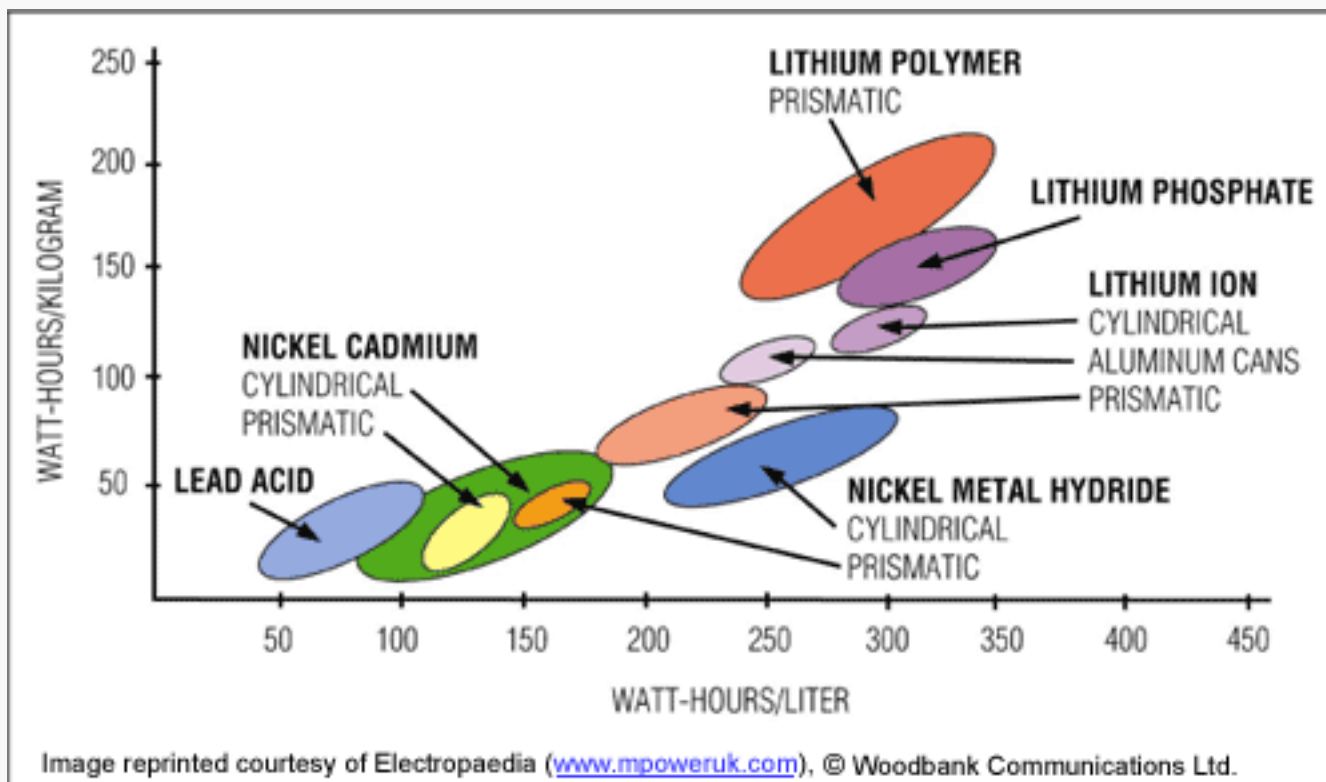
Figure 1. The energy densities of various battery types.
