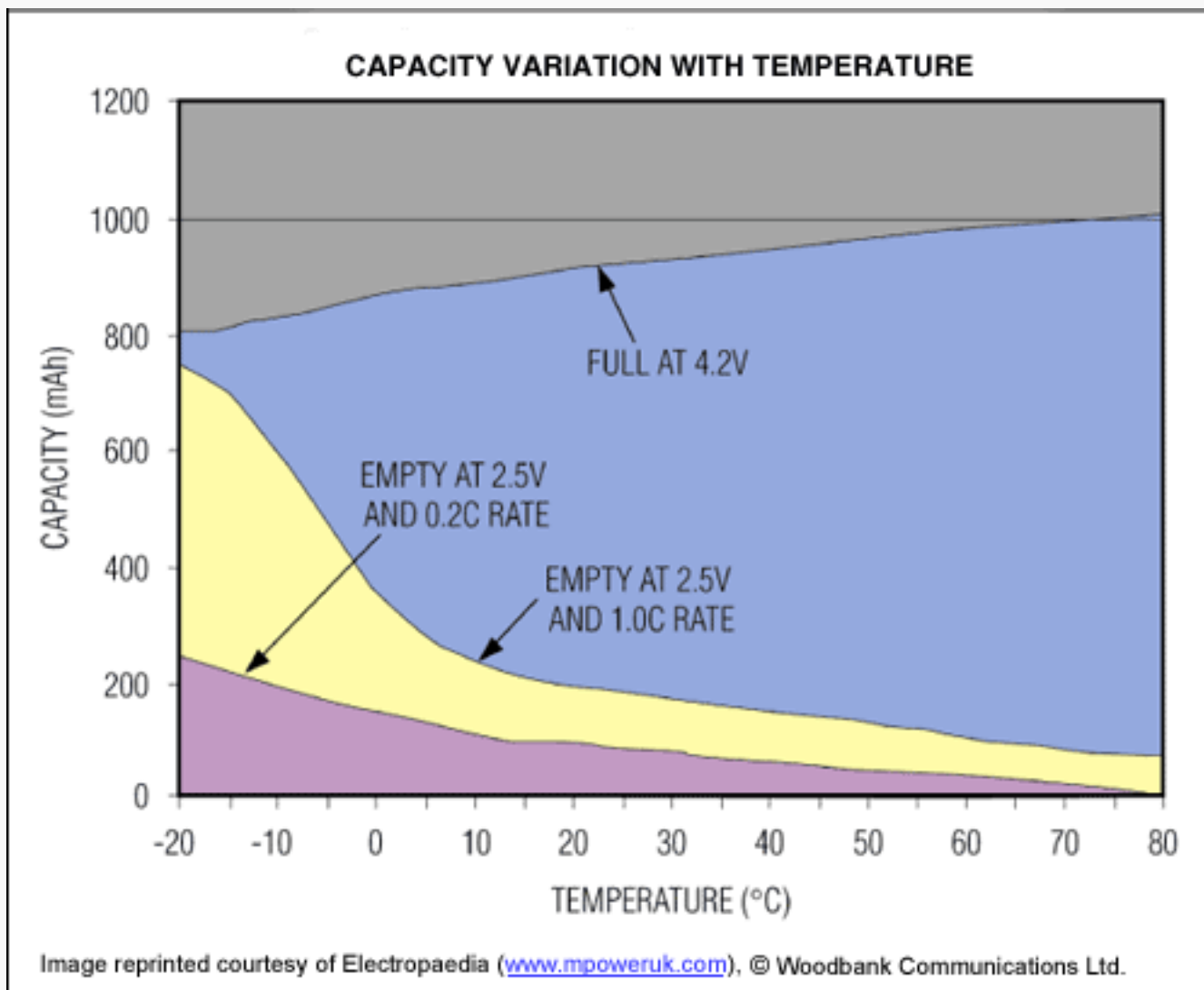
Figure 2. The influence of temperature on battery capacity.
