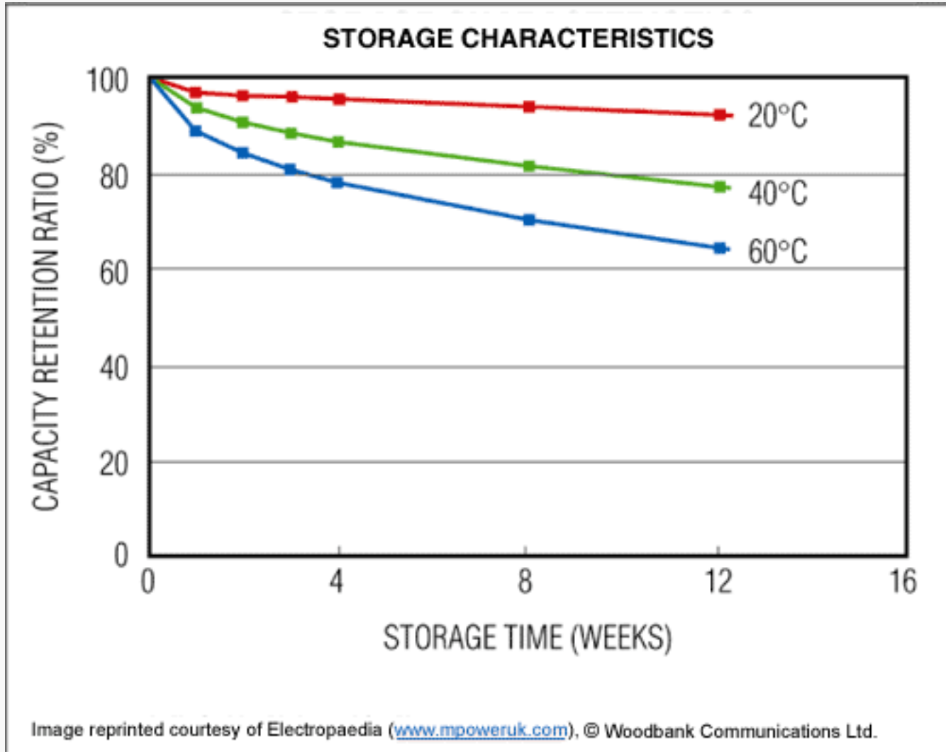
Figure 3. Self-discharge of Li-ion batteries.
