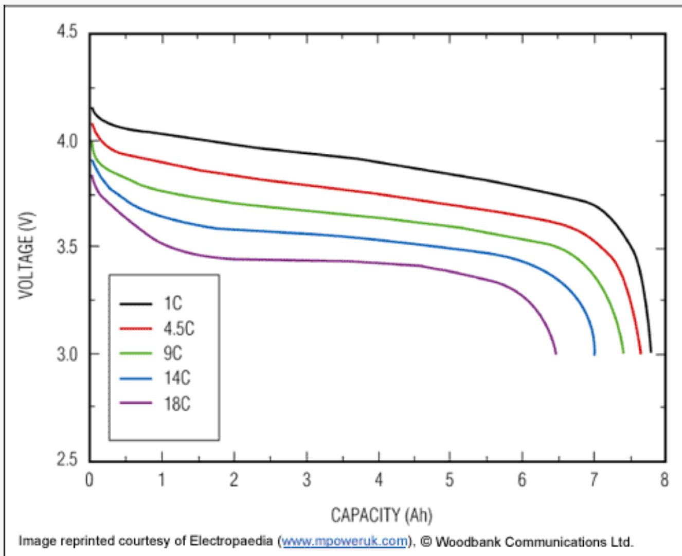
Figure 5. Battery-discharge curve.
