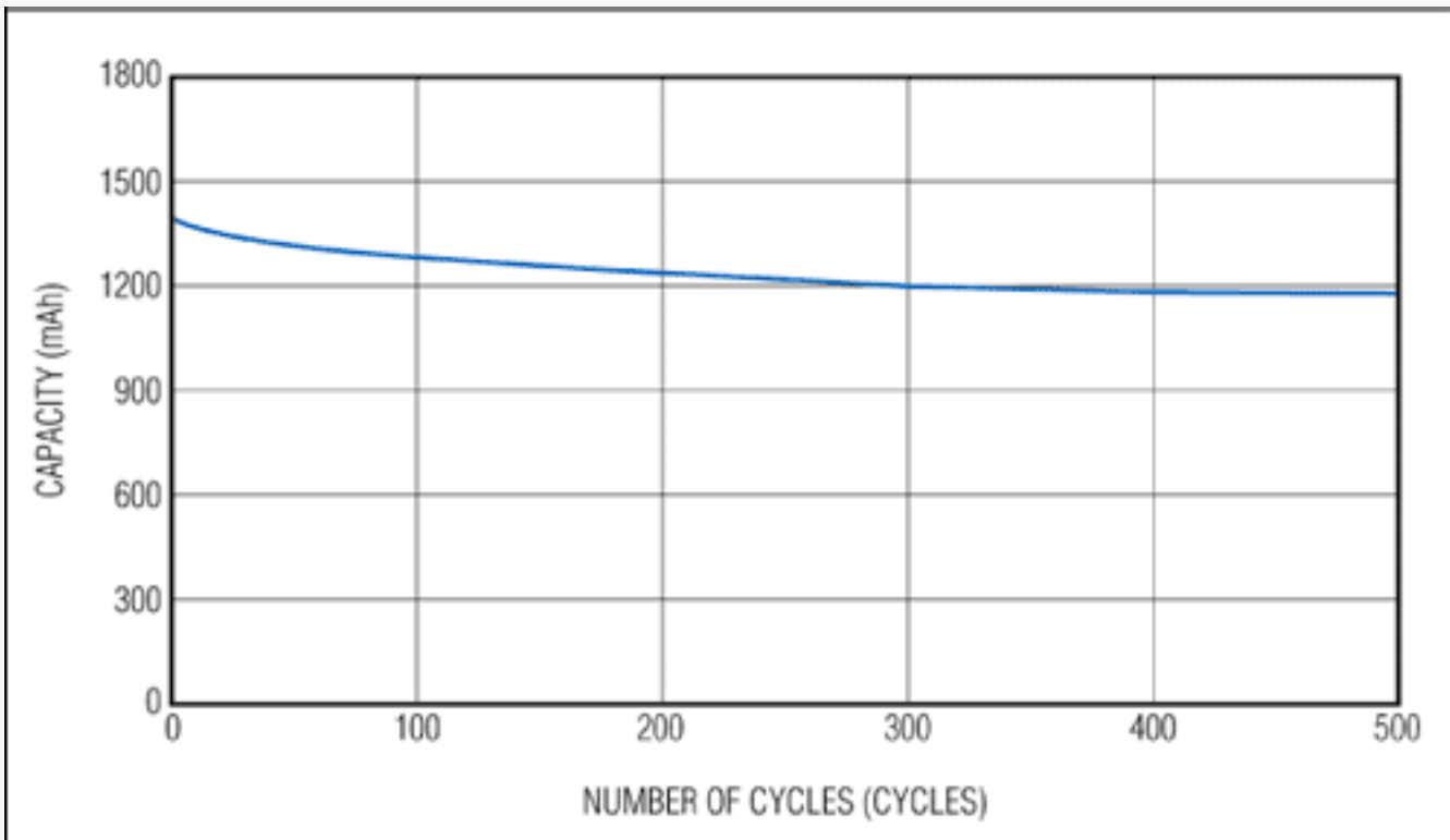
Figure 4. Battery aging.
