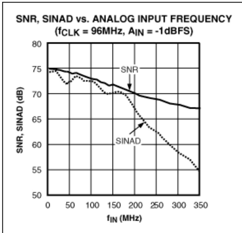
Figure 1. The SNR and SINAD for the 96Mps MAX12559 ADC are plotted vs. input frequency at a clock rate of 96MHz and an amplitude level of -1dBFS.
