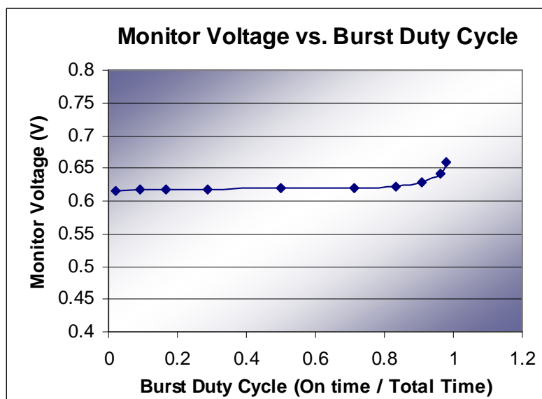
Figure 7. Monitor Voltage vs. Burst Duty Cycle
