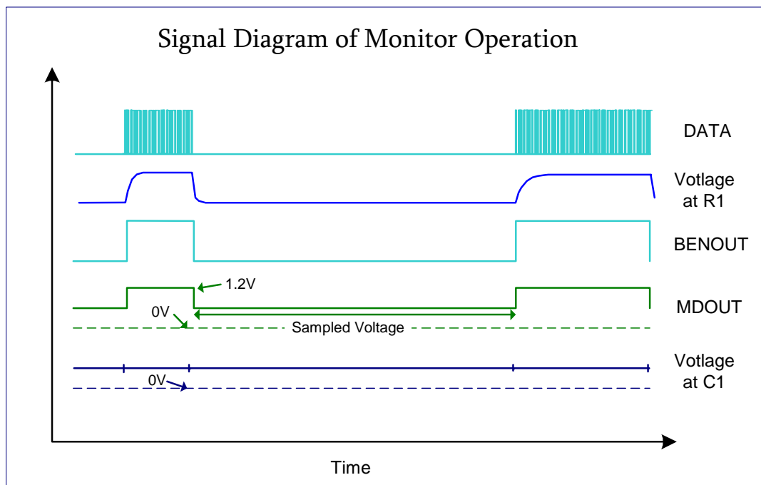
Figure 5. Monitor Diode Tracking (Burst Mode)
