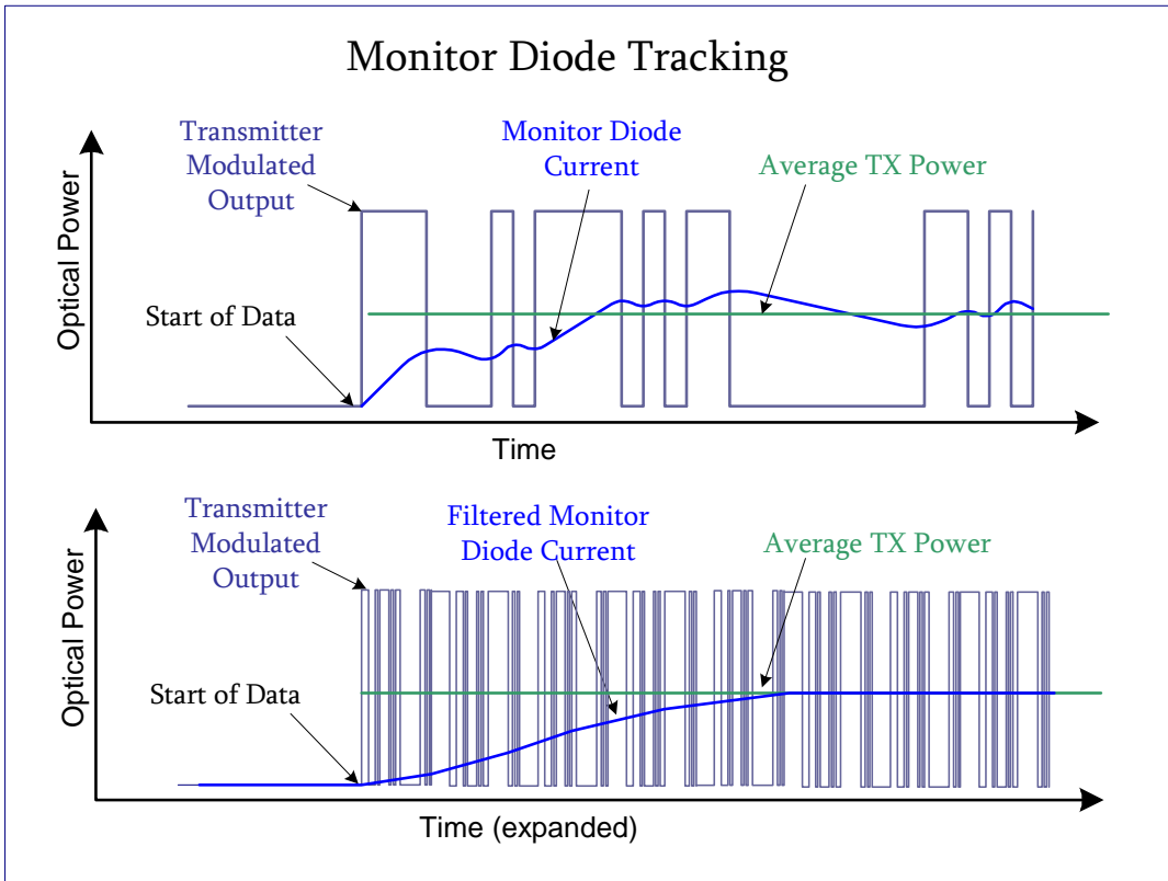
Figure 1. Monitor Diode Tracking
