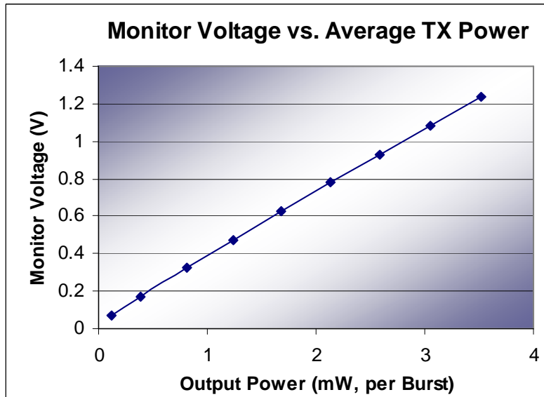
Figure 6. Monitor Voltage vs. Average TX Power
