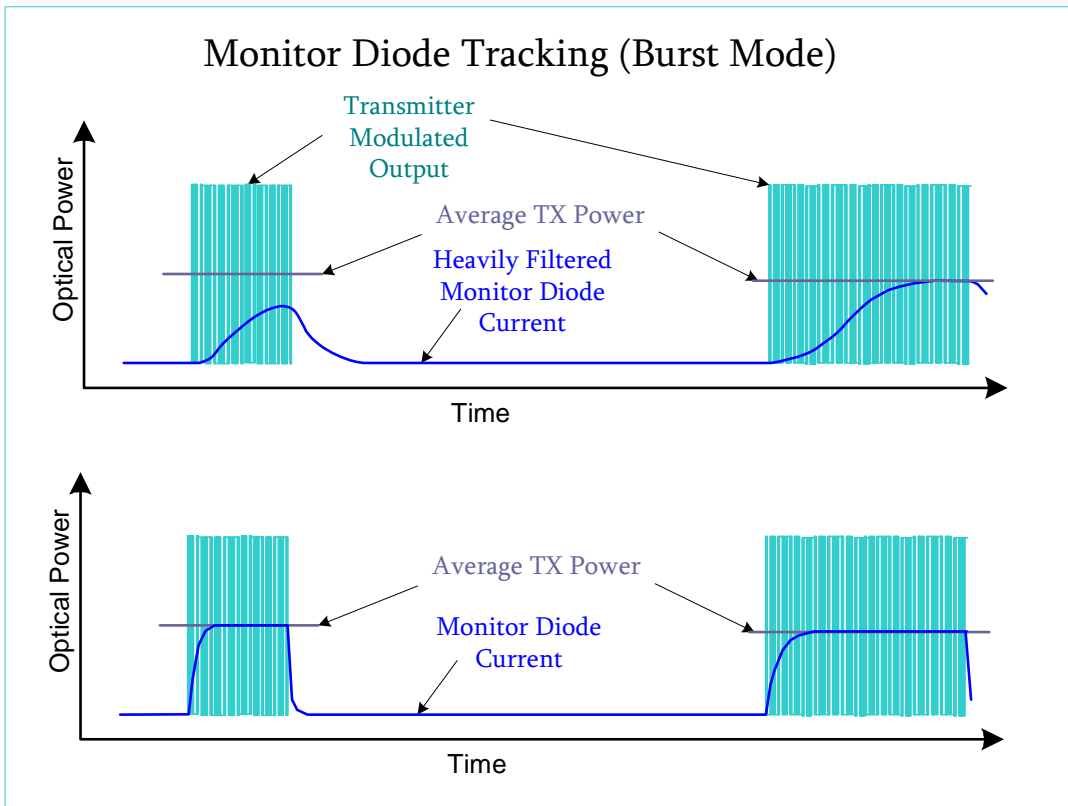
Figure 2. Monitor Diode Tracking (Burst Mode)
