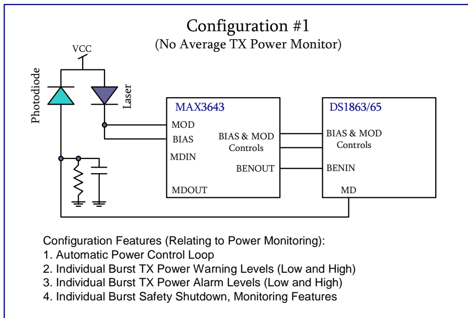
Figure 3. Configuration #1, No Average TX Power Monitor
