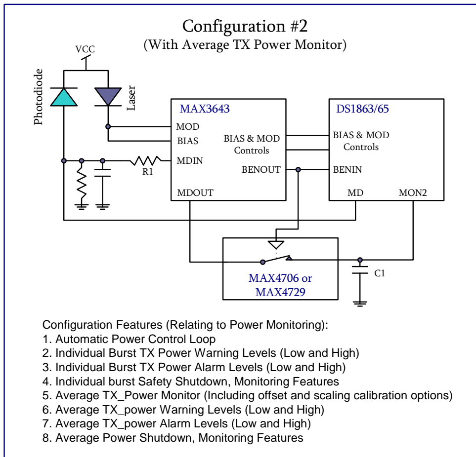
Figure 4. Configuration #2, Average TX Power Monitor
