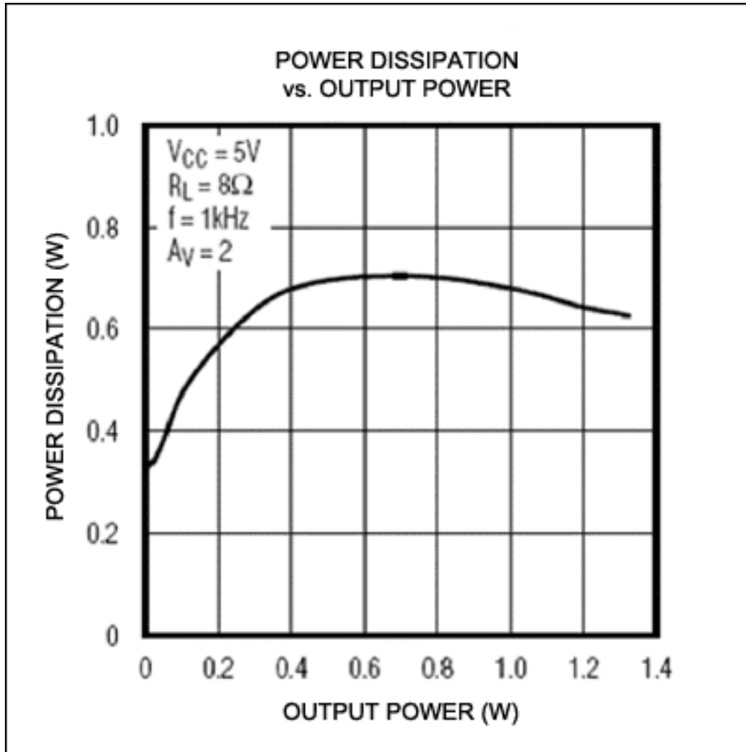
Figure 2. Power Dissipation vs. Output Power for a Class AB amplifier.
