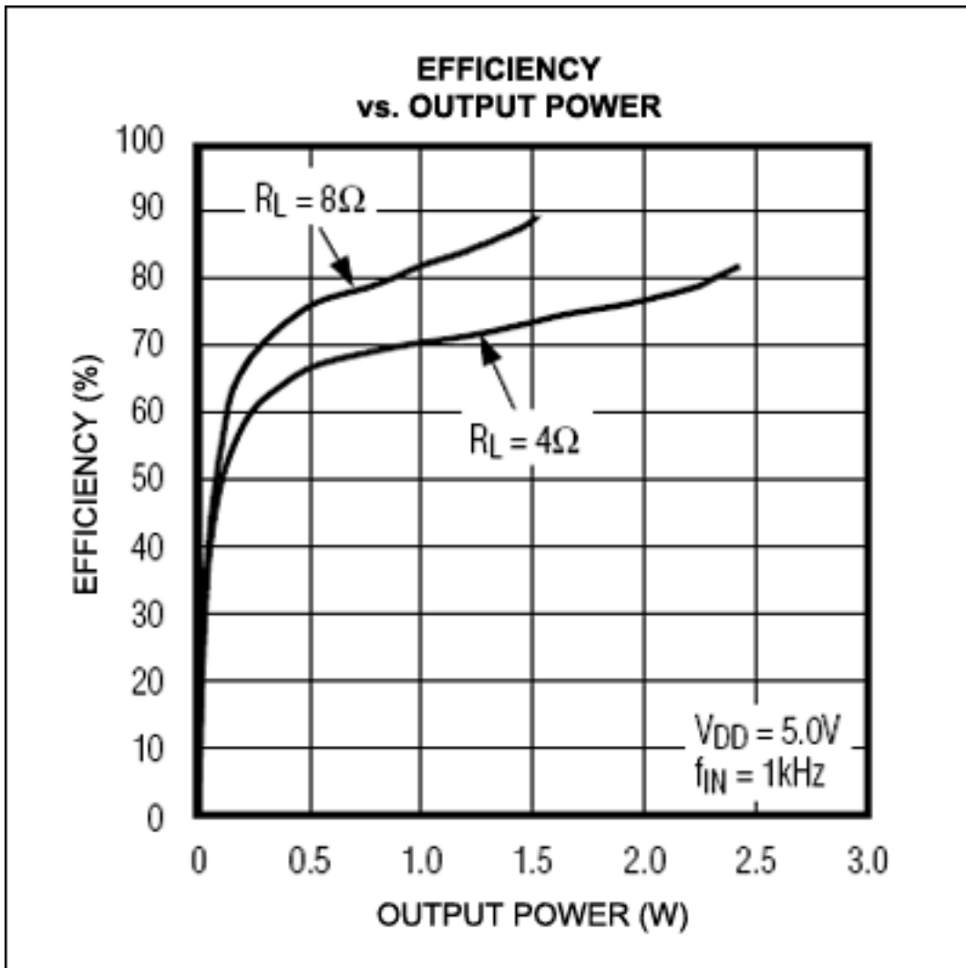
Figure 3. Efficiency vs. Output Power for a Class D amplifier.
