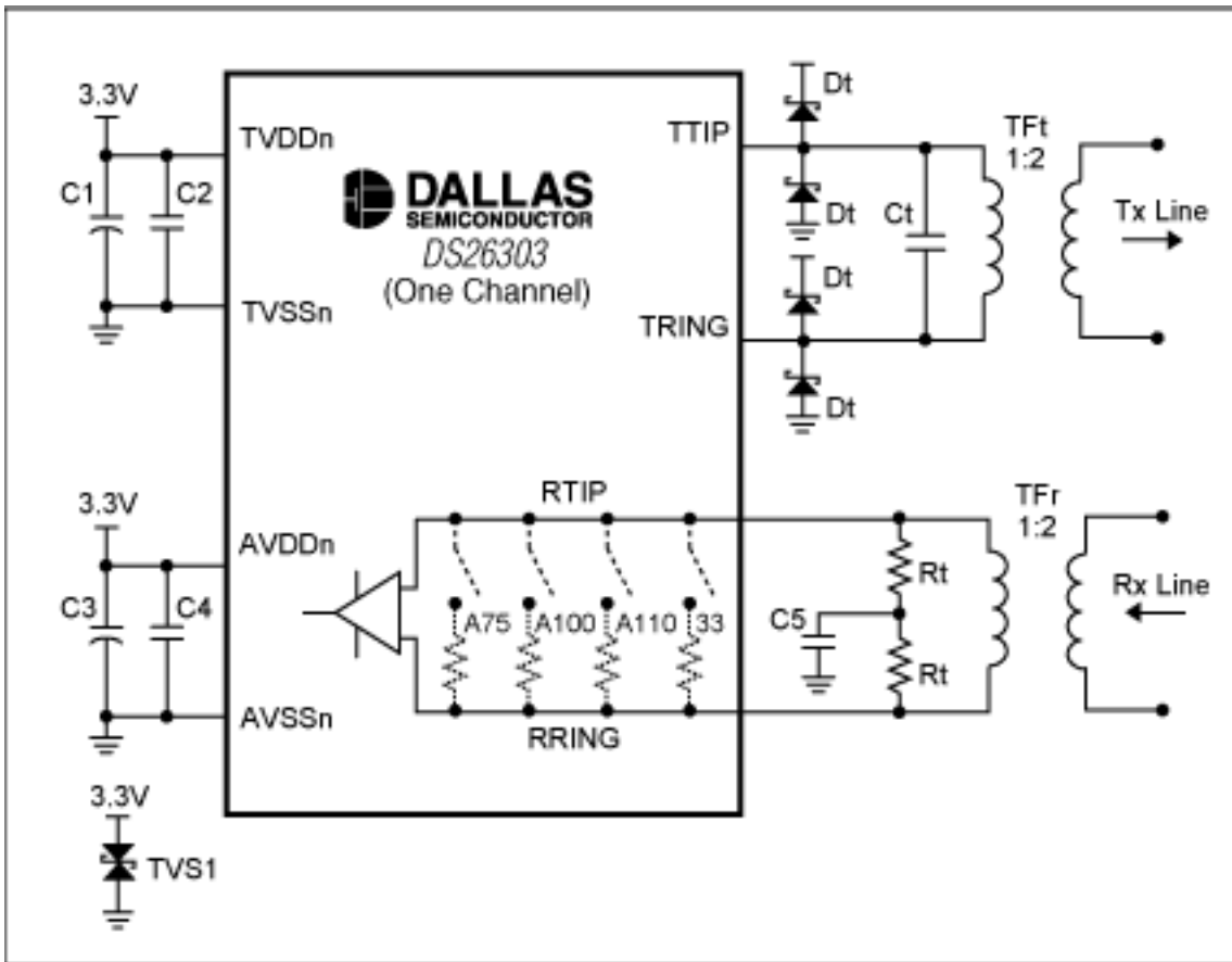
Figure 1. LIU front-end
