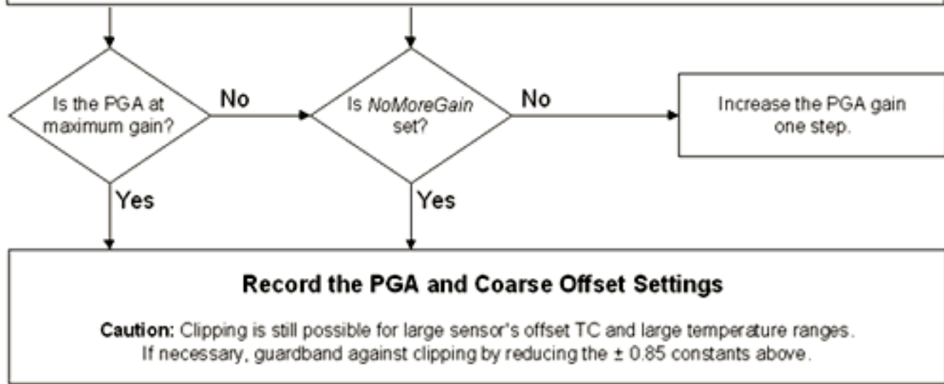
Figure 1. Procedure for determining the optimum Coarse Offset and PGA settings for compensating a sensor signal using the MAX1464 signal conditioner.
