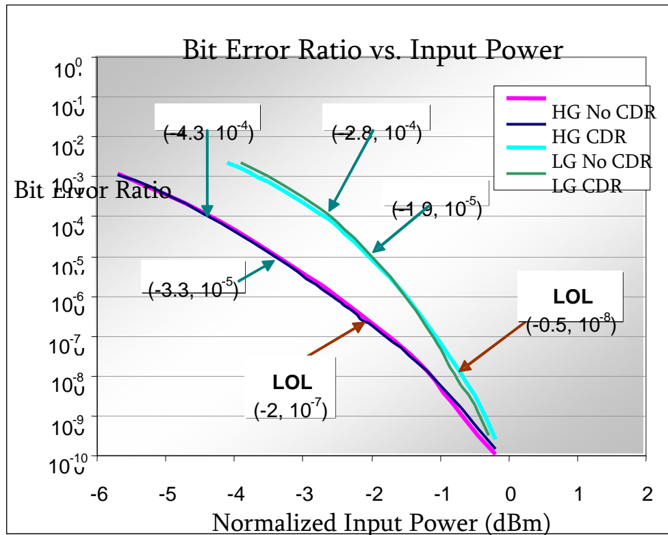
Figure 2: Bit Error Ratio vs. Input Power
