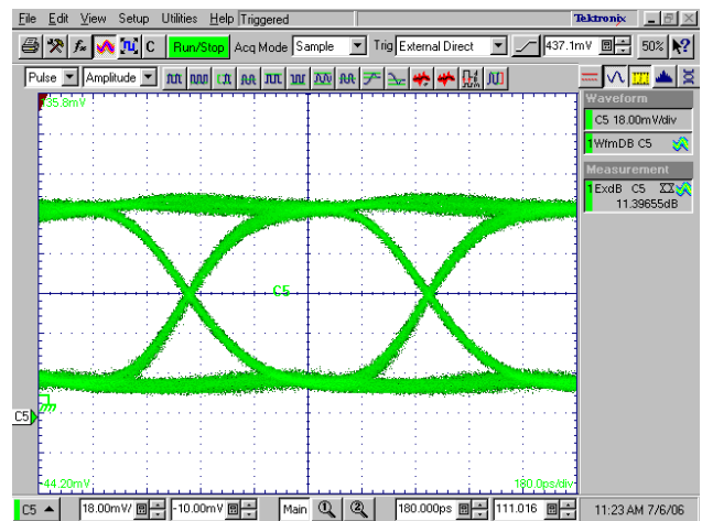
Figure 16. Room Temp, VCC = 3.0V
