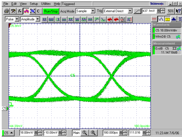
Figure 17. Room Temp, VCC = 3.3V
