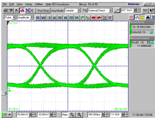
Figure 13. Eye Diagram, Temp = +40°C
