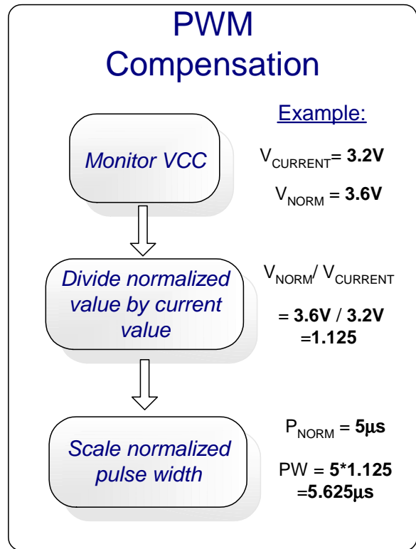
Figure 7. PWM Compensation
