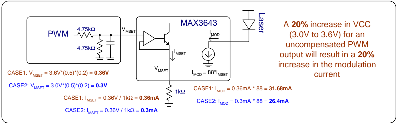
Figure 6. VCC Variation
