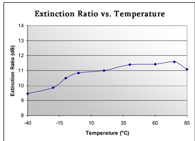
Figure 11. Extinction Ratio (-40°C to 85°C)
