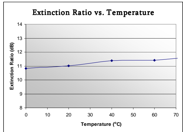
Figure 10. Extinction Ratio (0°C to 70°C)
