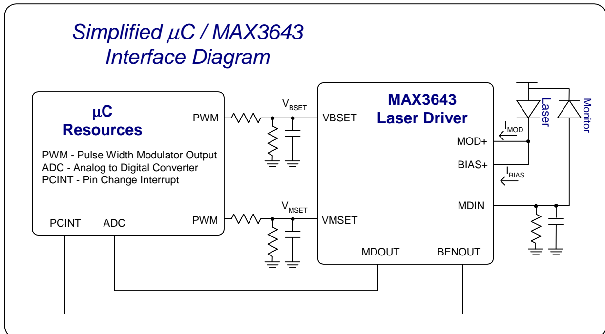
Figure 3. Simplified \mu\text{C} / MAX3643 Interface Diagram
