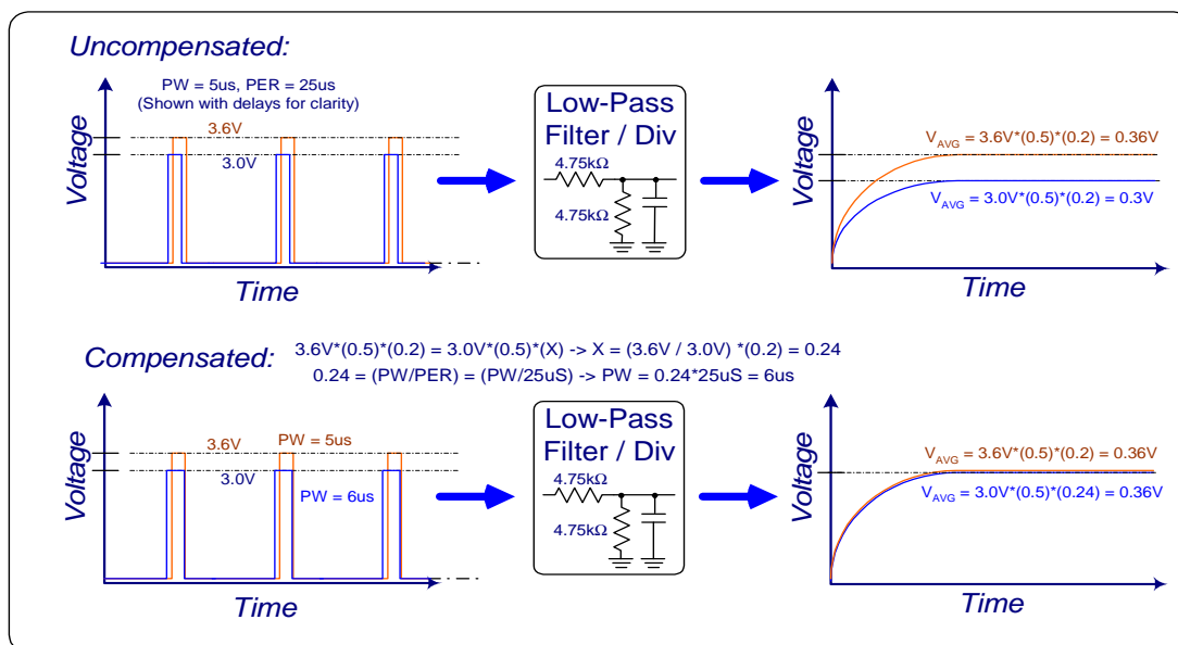
Figure 5. Uncompensated vs. Compensated PWM
