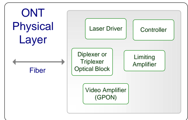
Figure 2. Typical ONT Physical Layer
