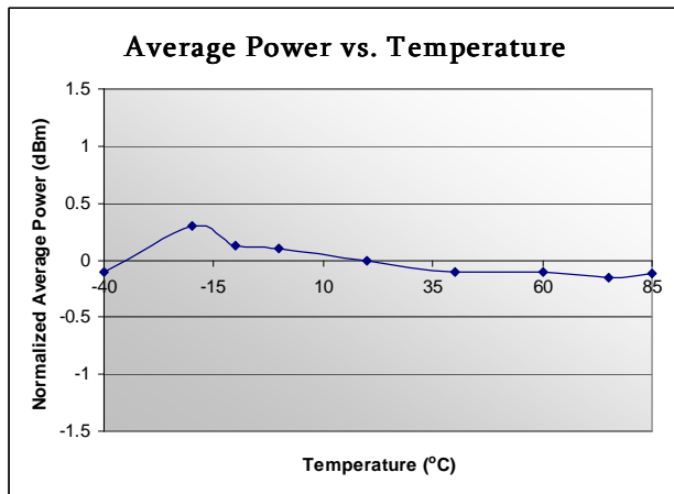
Figure 9. APC Loop Performance
