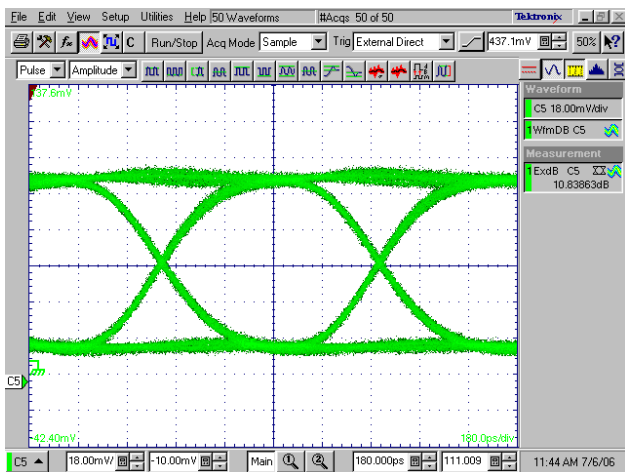
Figure 14. Eye Diagram, Temp = 0°C
