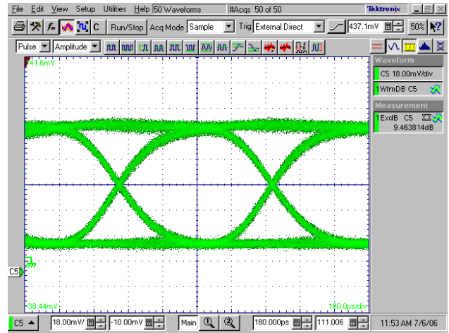
Figure 15. Eye Diagram, Temp = -40°C
