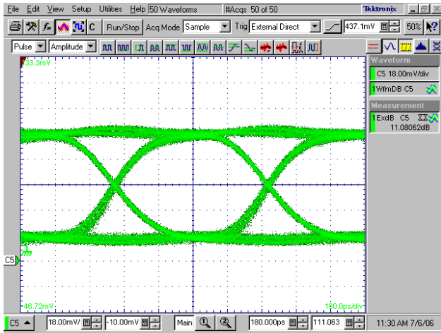
Figure 12. Eye Diagram, Temp = +85°C
