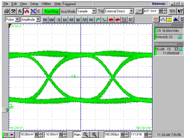
Figure 18. Room Temp, VCC = 3.6V
