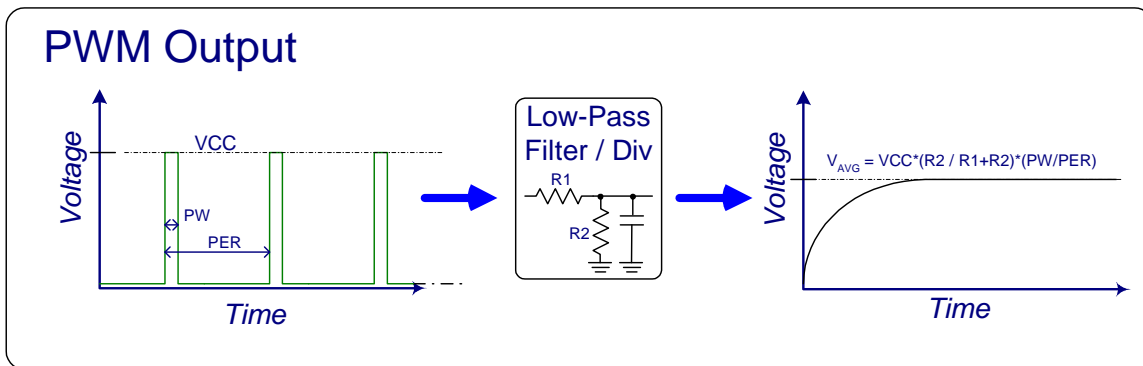
Figure 4. PWM Output to DC voltage conversion
