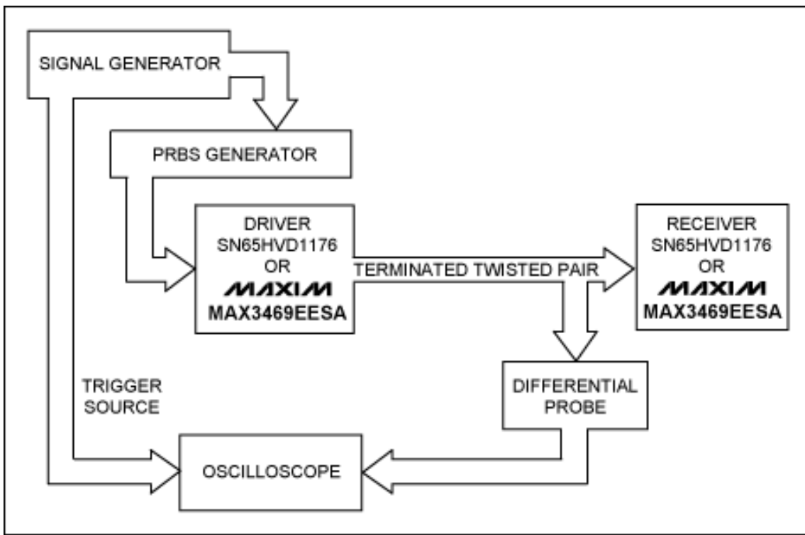
Figure 1. Test setup.
