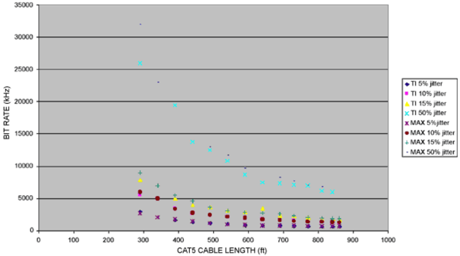
Figure 4. Graph of jitter for a given bit rate and cable length. Jitter is measured at \pm 100\text{mV} differential.
