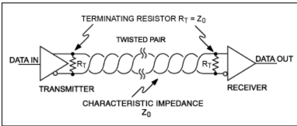
Figure 7. Single transmit, single receive network.
