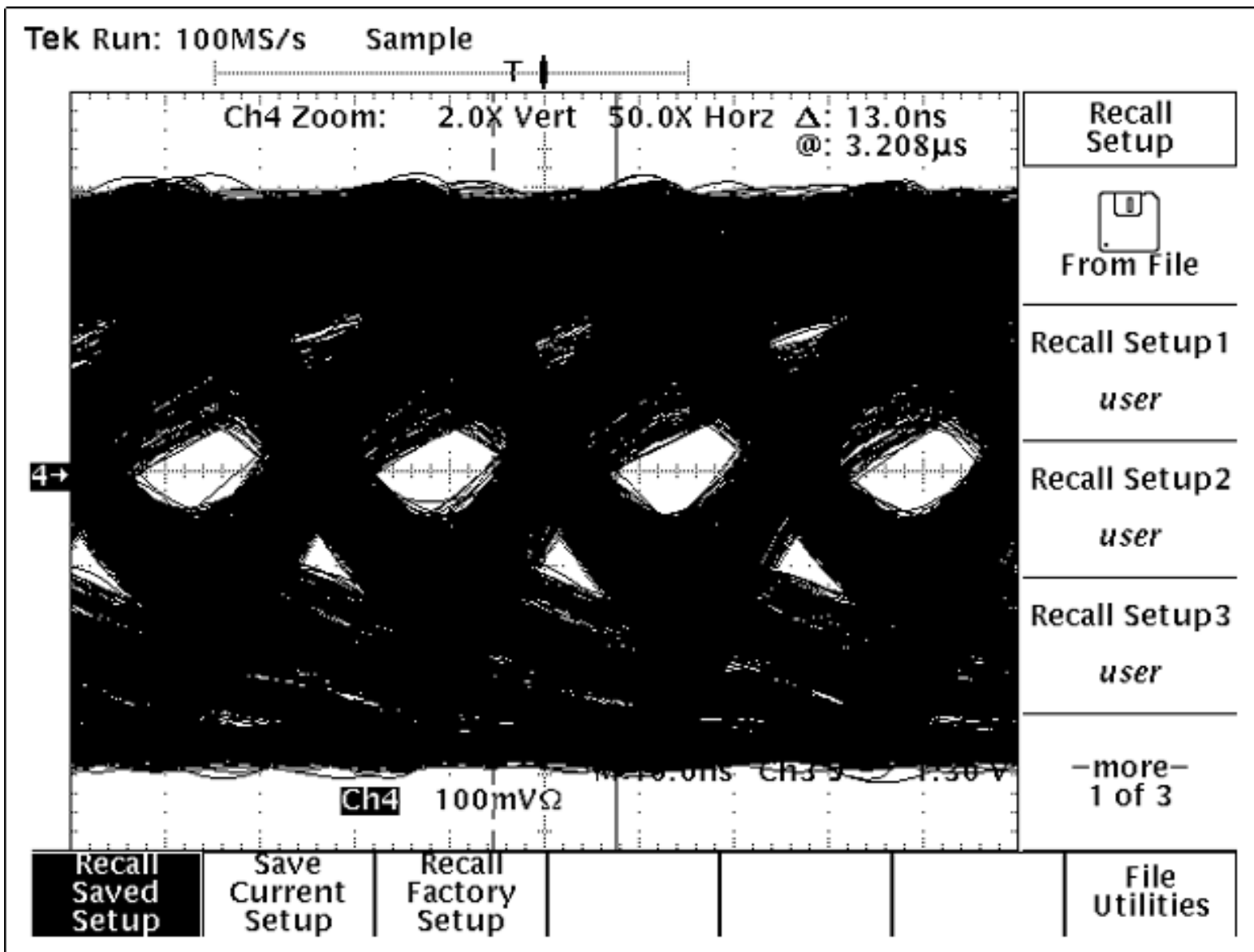
Figure 3. Eye pattern for Maxim's MAX3469.
