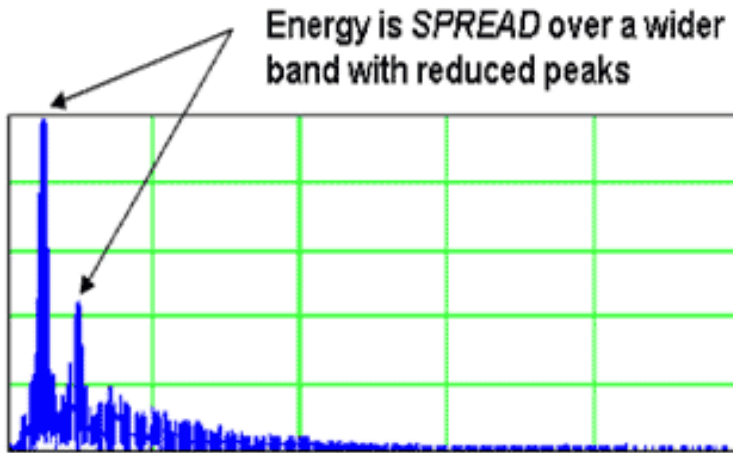
Figure 5b. Maxim's Spread-Spectrum-Modulation Mode.
