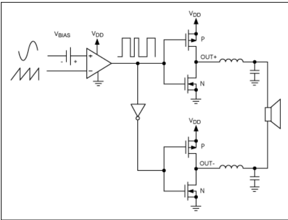
Figure 1. Conventional Pulse-Width-Modulation Topology.
