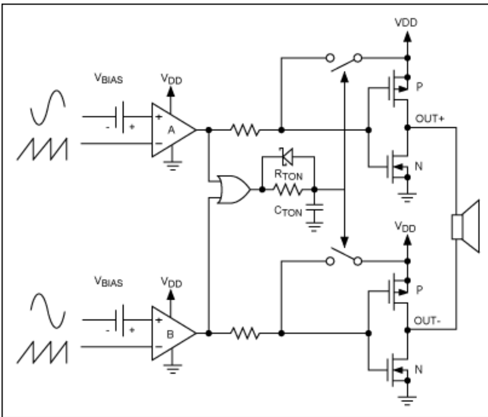
Figure 2. Mono Class D Amplifier Topology.
