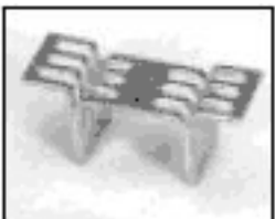
Figure 4. An SMT heatsink, such as the one pictured here, may be needed when a Class D amplifier is operated at higher ambient temperatures. (Photo courtesy of Wakefield Engineering.)
