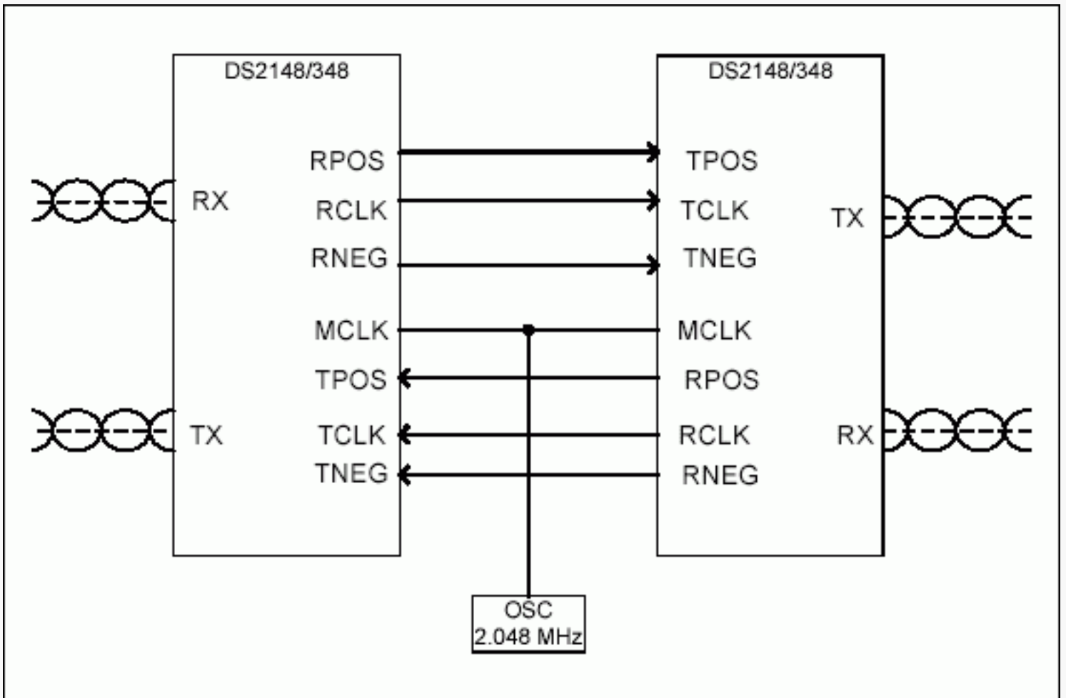
Figure 1. Typical T1/E1 repeater application.
