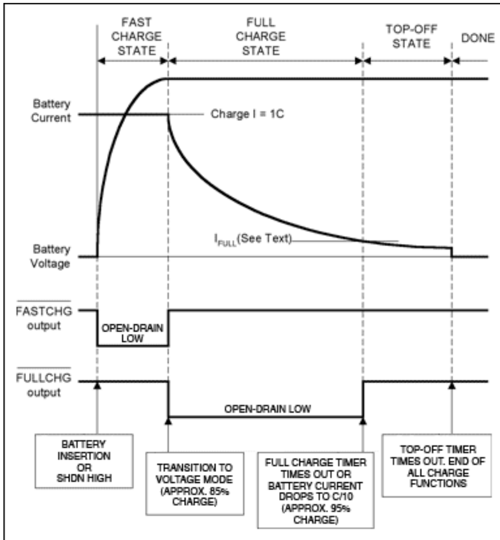
Figure 2. Charge state and indicator timing for a typical charging sequence. Full battery is indicated when FULLCHG-bar goes high with FASTCHG-bar already high. This occurs when battery charging current falls to I_{FULL} , as described in the text.
