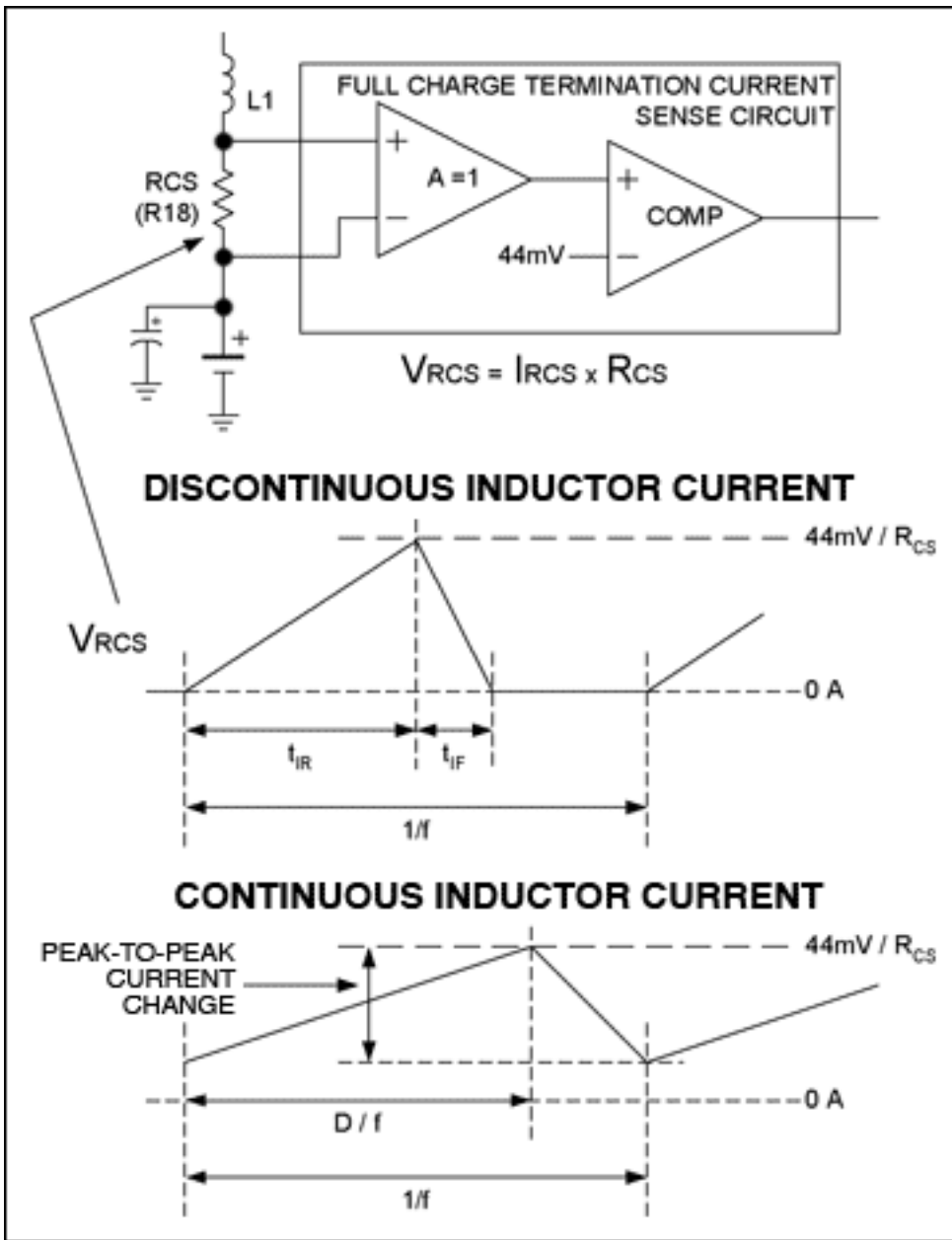
Figure 1. Full-charge termination detection circuit and inductor current waveforms. Full charge is indicated when peak inductor current falls below 44\text{mV}/R_{CS} . The battery charging current that corresponds to this peak current is a function of inductor value and input voltage, and can be calculated as described in the text.
