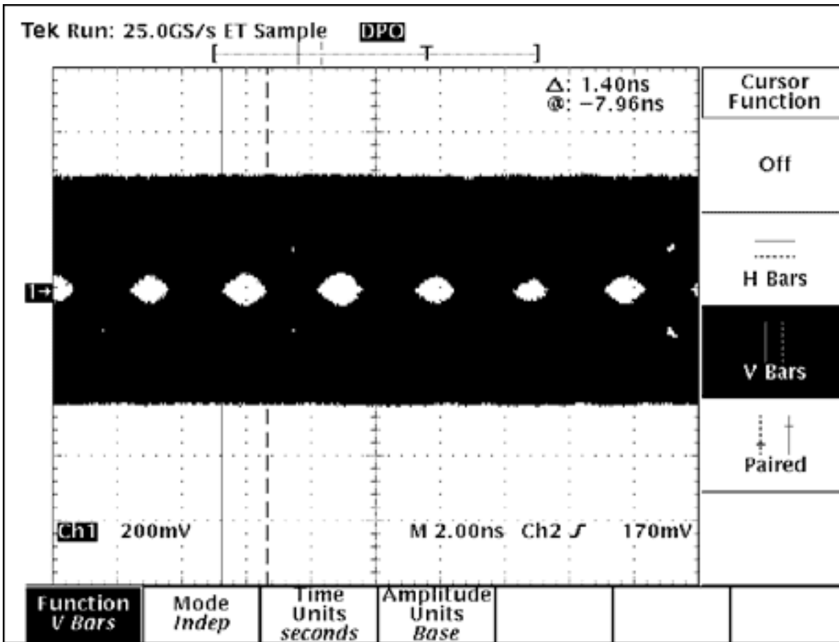
Figure 5. NISSEI AWG26, 30m at 306Mbps with pre-emphasis.
