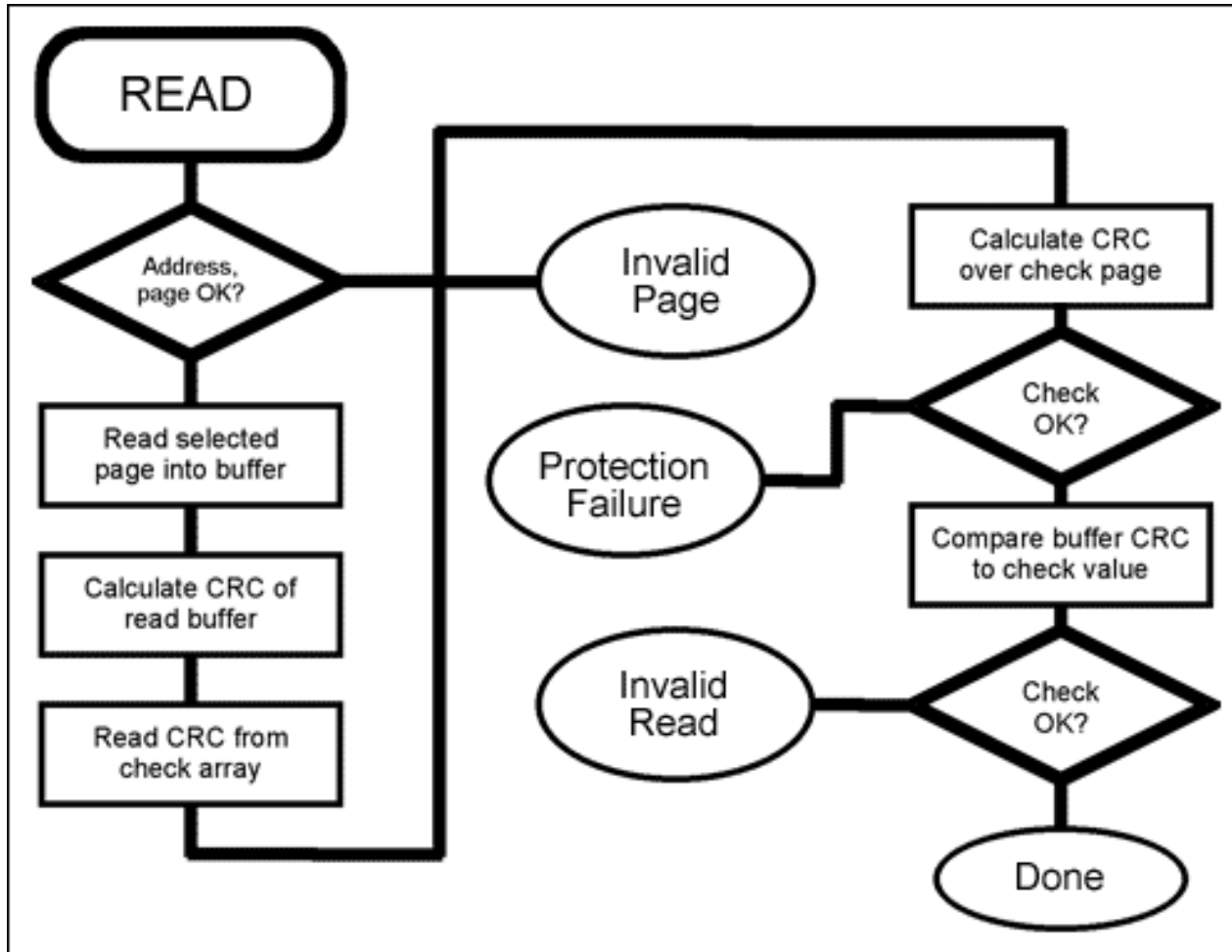
Figure 2. Flowchart for a READ operation.
