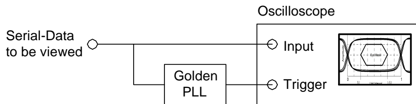
Figure 8. Viewing jitter using a sampling scope
