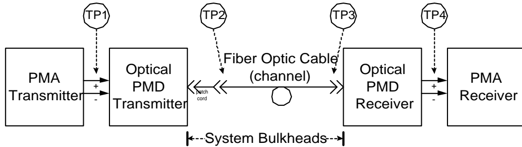
Figure 5. Serial link using fiber optic cabling
