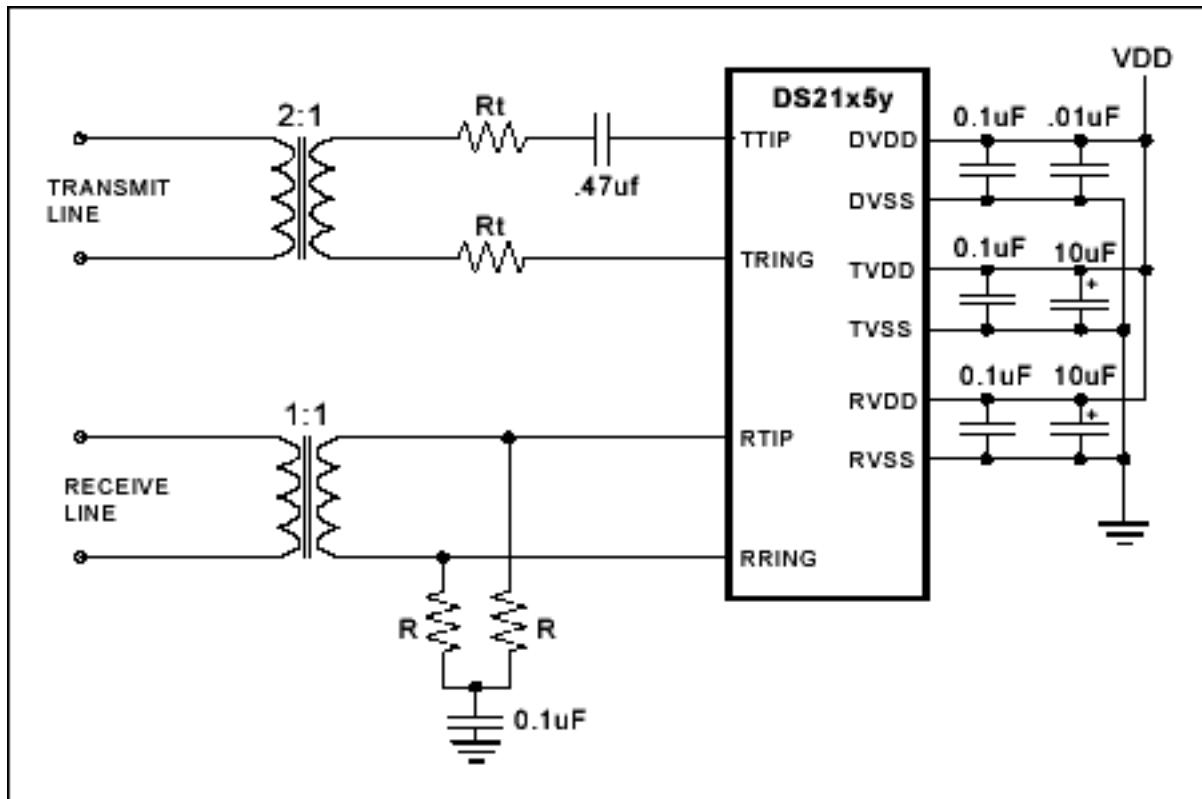
Figure 2. DS21x5y network interface.
