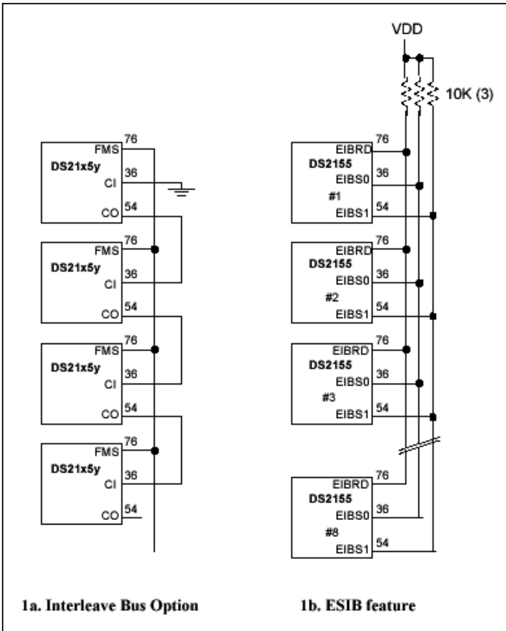
Figure 1. Pins 36, 54 and 76 usage.
