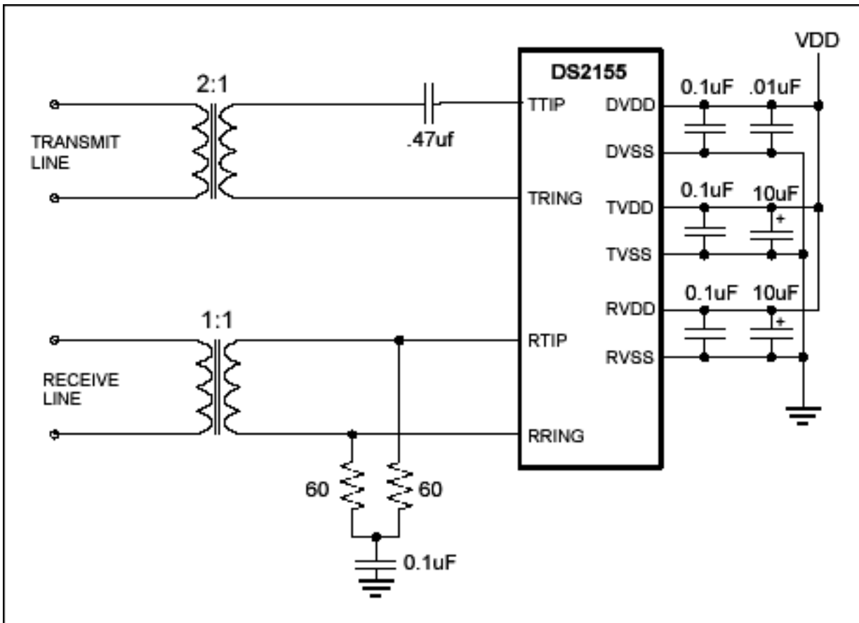
Figure 3. DS2155 network interface.
