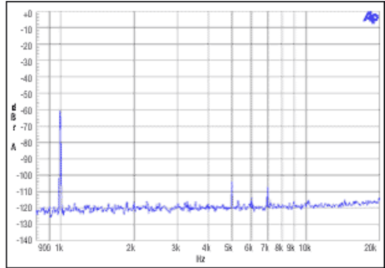
Figure 7. Master/slave integer mode. MCLK = 12.288MHz , F_S = 48kHz , -30dBFS and -60dBFS.
