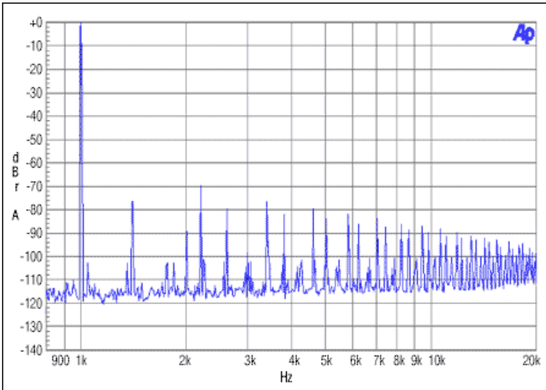
Figure 6. Slave noninteger mode. MCLK = 12\text{MHz} , F_S = 44.1\text{kHz} , 0\text{dBFS} .
