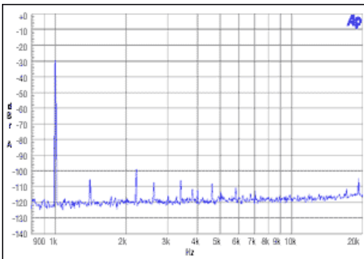
Figure 11. Slave noninteger mode. MCLK = 12MHz , F_S = 44.1kHz , -30dBFS , -60dBFS .
