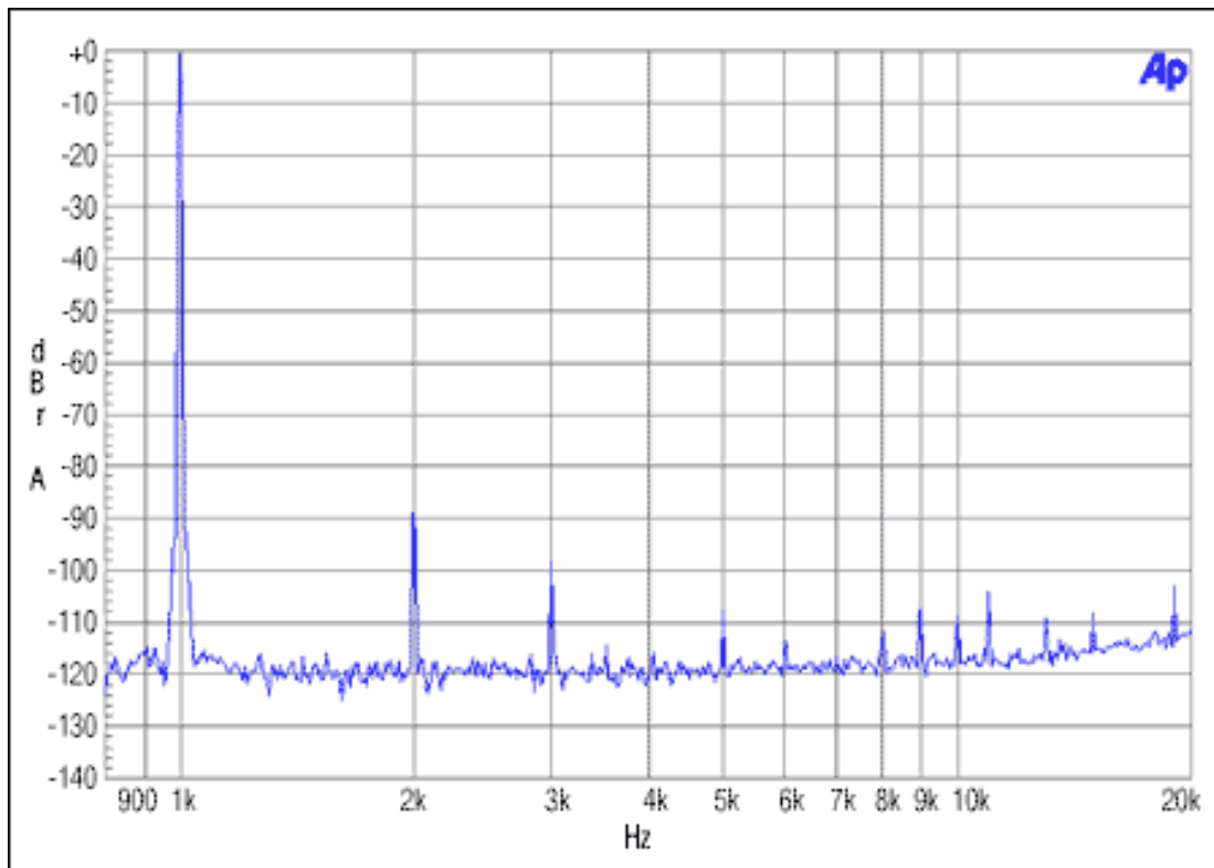
Figure 1. Master-integer mode. MCLK = 12.288MHz, F_S = 48\text{kHz} , 0dBFS.
