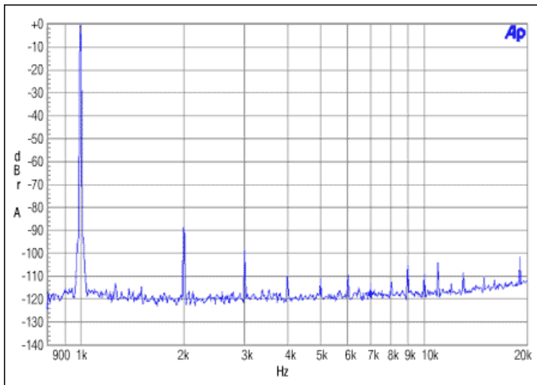
Figure 2. Slave-integer mode. MCLK = 12.288MHz , F_S = 48kHz , 0dBFS .
