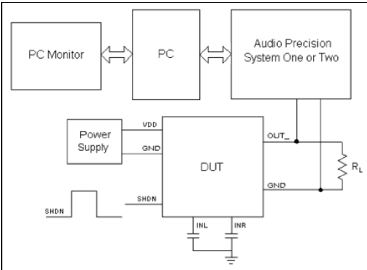
Figure 3. Test setup for click-and-pop measurements in headphone amplifiers. Note that the left and right input pins are AC-coupled to ground. The outputs are loaded with typical headphone impedance and the shutdown pin is toggled by a square wave generator.
