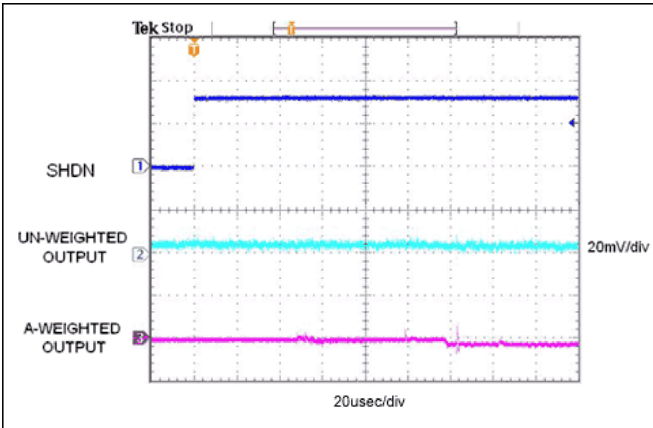
Figure 2. Data show the transient events associated with a low-offset, DC-coupled headphone amplifier brought out of shutdown. The amplitude is much lower in comparison to Figure 1 (hence subjectively quieter), and the amplifier is fully enabled after 150 \mu s.
