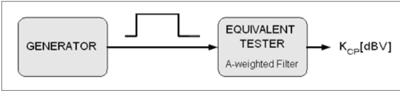
Figure B. Test setup for calibration of equivalent audio analyzers. Calibration must be performed to ensure that the amount of energy recorded by the equivalent analyzer is linear with the varying input amplitude.
