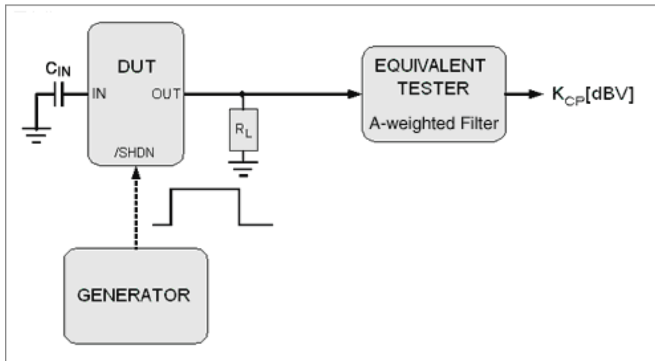
Figure A. A test setup for click-and-pop measurements using equivalent test equipment from other manufacturers.
