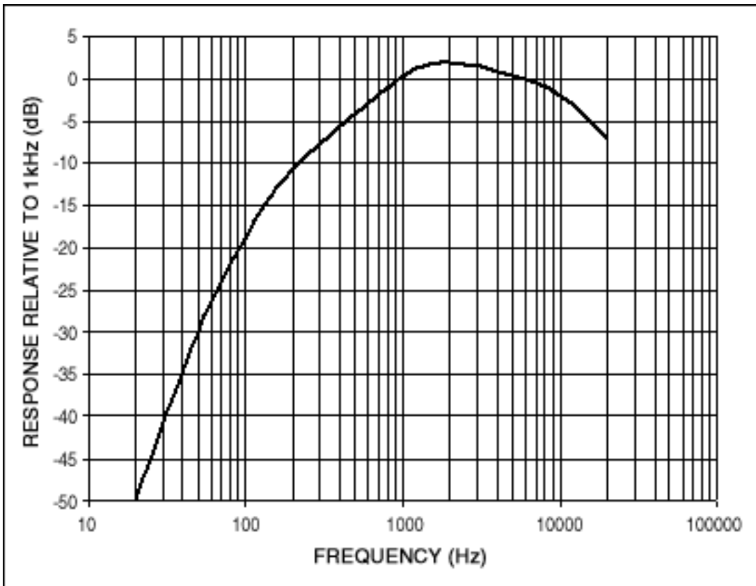
Figure 4. Frequency response of the A-weighted filter. This parameter is often used for noise measurements, as the frequency balance approximates the ear's sensitivity. Note that the filter transfer function is unity gain (0dB) at 1kHz, and attenuates the frequency extremes.
