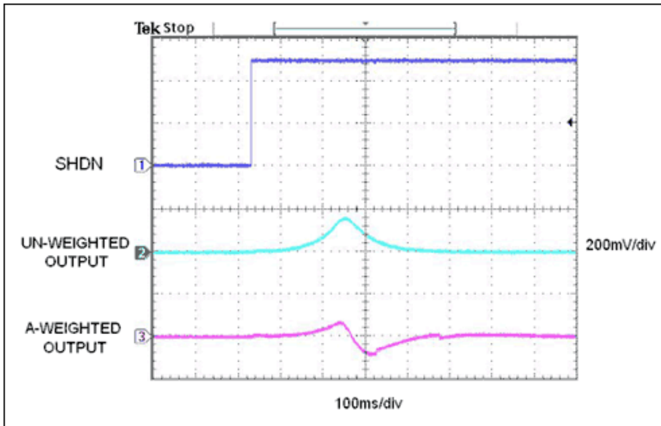
Figure 1. Data show the transient events associated with a particularly well-behaved, AC-coupled headphone amplifier brought out of shutdown. Although high in amplitude, this transient will produce a predominantly low-frequency sound, to which the ear is less sensitive.
