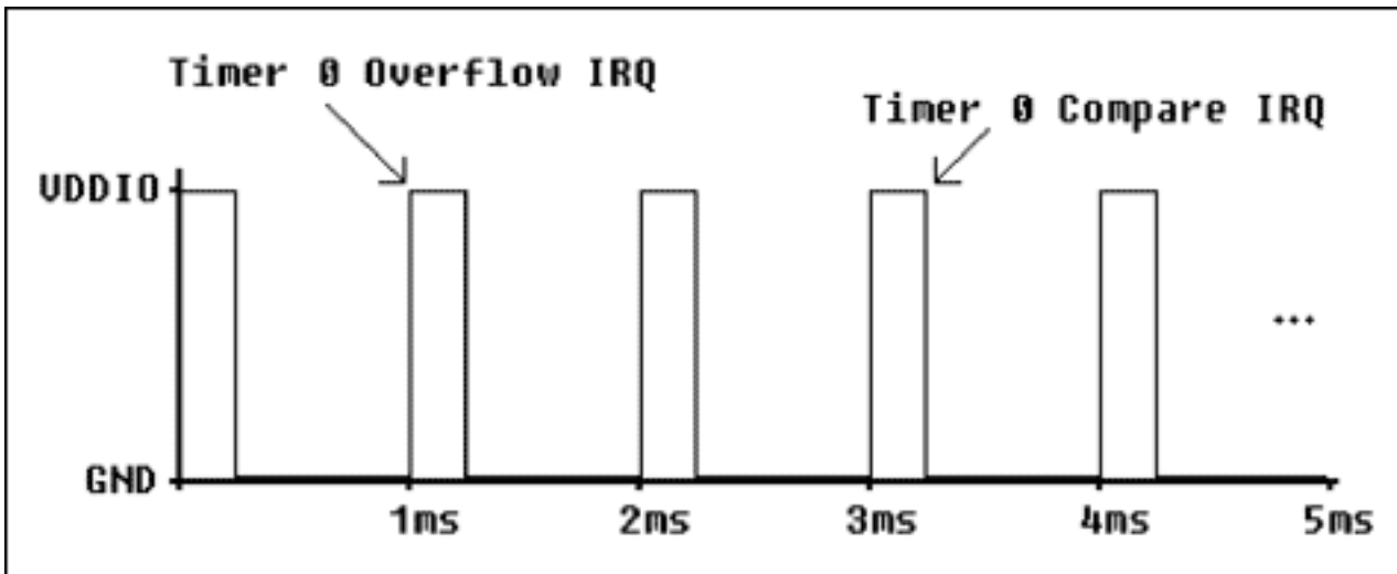
Figure 1. Using Timer 0 to generate a PWM signal.
