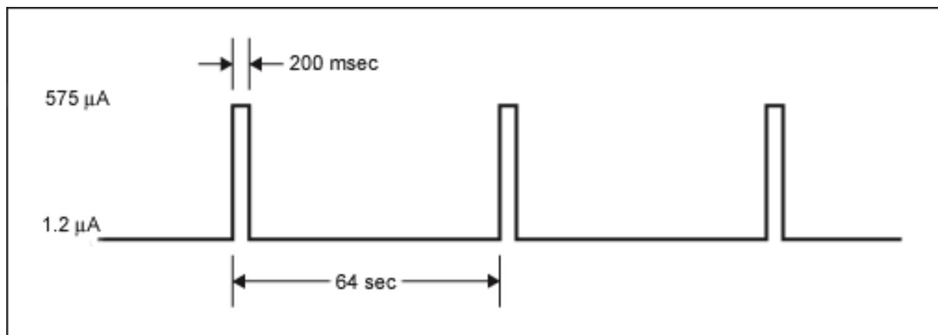
Figure 1. DS3231 Worst-case current requirements.
