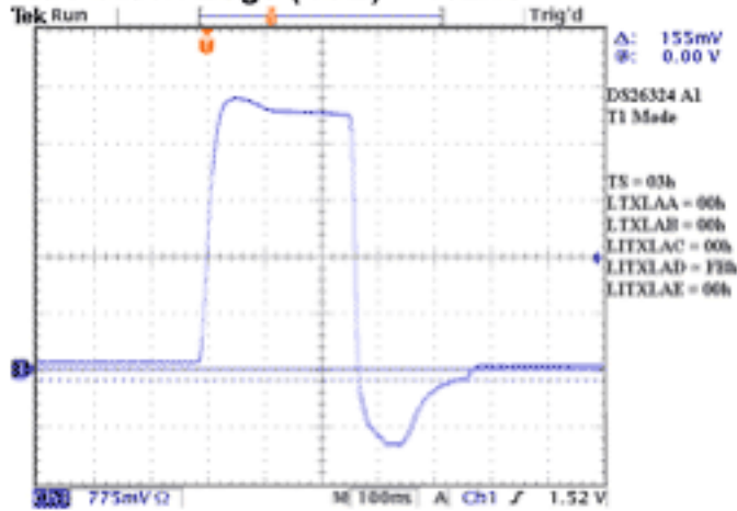
T1 Min Undershoot (4) Max (4CE)
