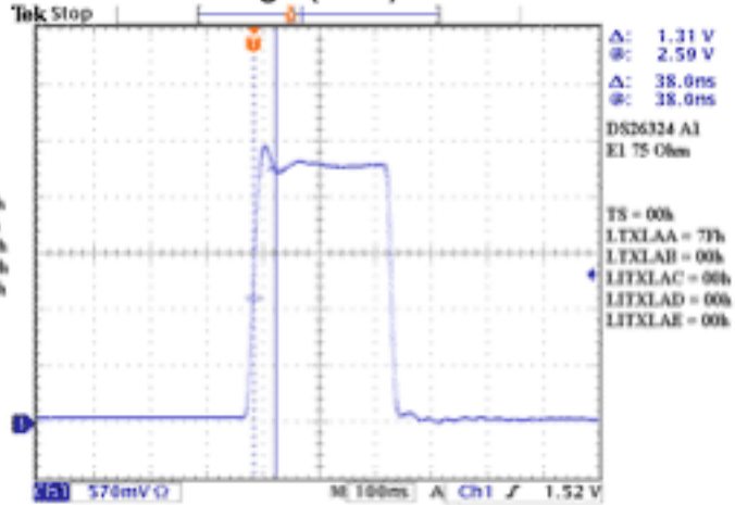
E1 75 Max Overshoot (1) Min (1CE)
