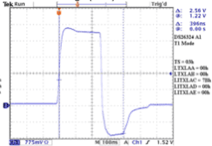
T1 Max Undershoot (3) Max (3CE)
