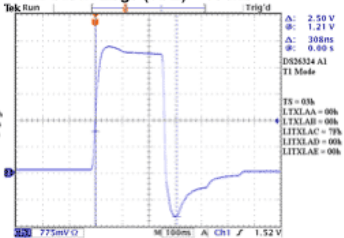
T1 Max Undershoot (3) Min (3CE)
