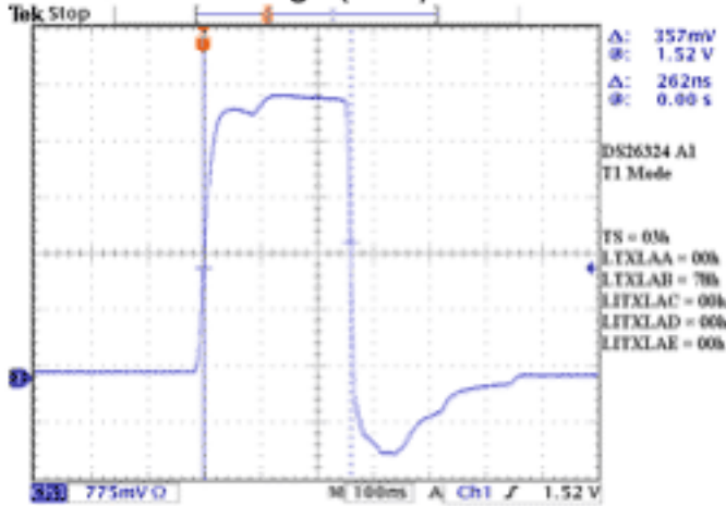
T1 Max Plateau (2) Normal (2CE)
