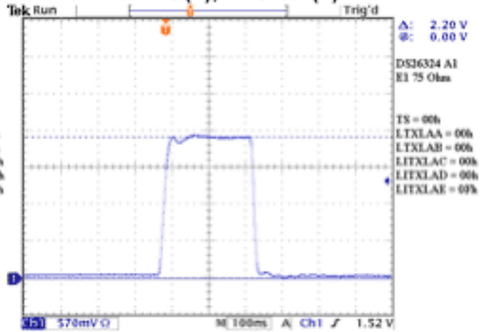
E1 75 Min DAC No Overshoot (1) Plateau (2)
