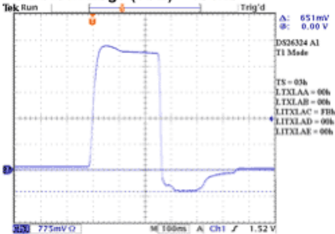
T1 Min Undershoot (3) Max (3CE)
