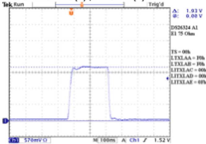
E1 75 Min DAC Min Overshoot (1) Plateau (2)
