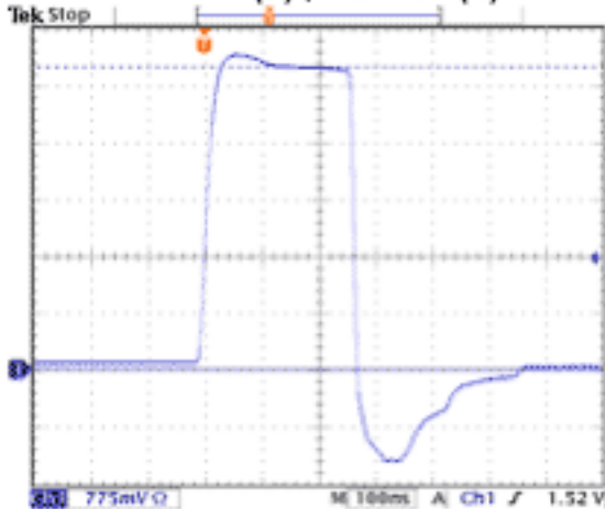
T1 Max DAC No Overshoot (1) Plateau (2)
