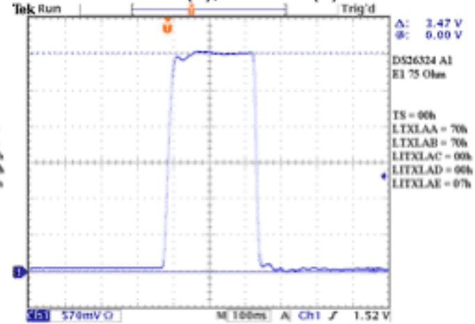
E1 75 Max DAC Max Overshoot (1) Plateau (2)
