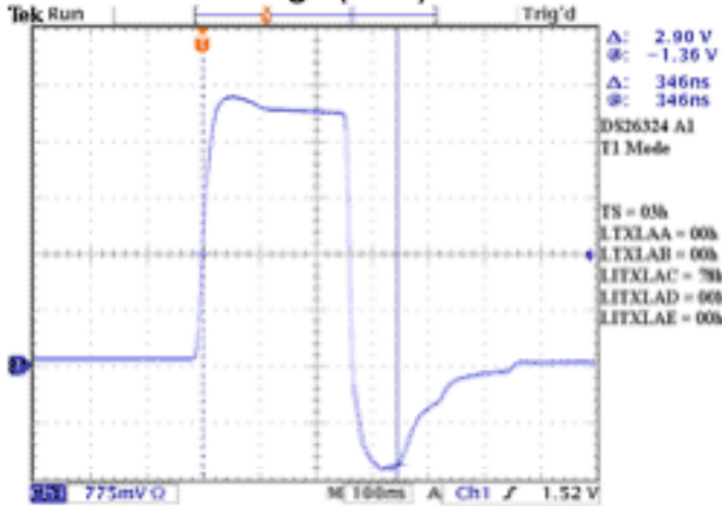
T1 Max Undershoot (3) Norm (3CE)
