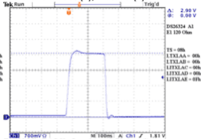
E1 120 Min DAC No Overshoot (1) Plateau (2)
