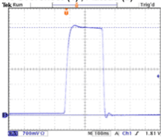
E1 120 Max DAC No Overshoot (1) Plateau (2)
