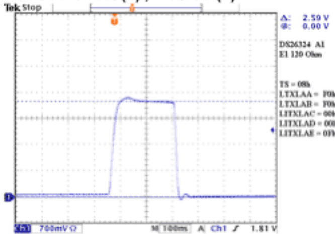
E1 120 Min DAC Min Overshoot (1) Plateau (2)
