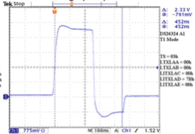
T1 Max Undershoot (4) Max (4CE)
