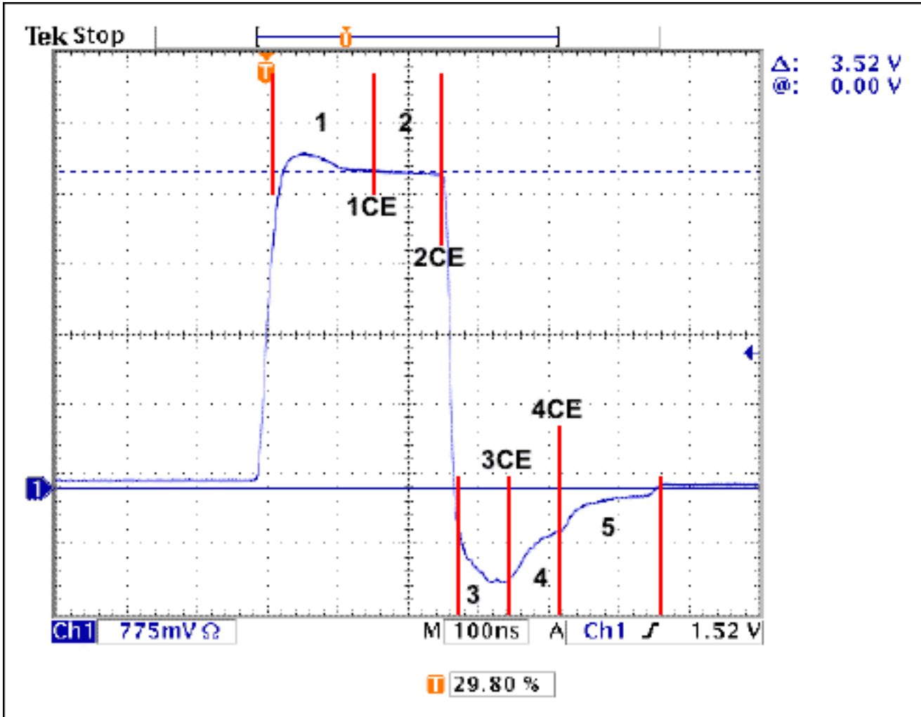
Figure 1. T1 pulse control sections.
