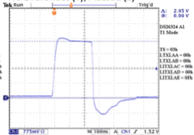
T1 Min DAC No Overshoot (1) Plateau (2)
