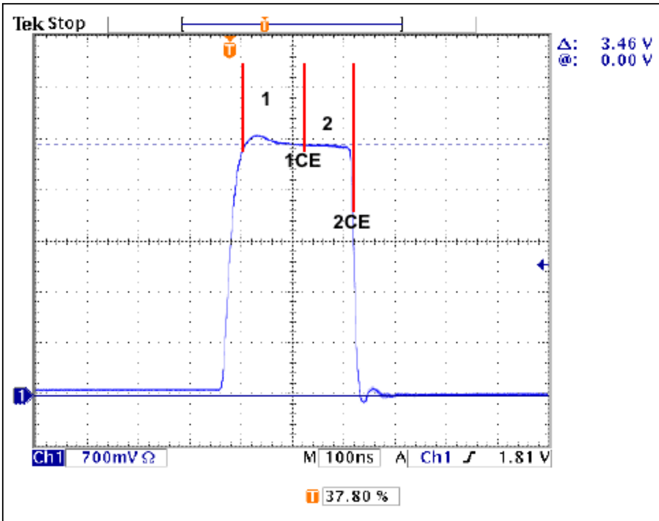
Figure 2. E1 pulse control sections.
