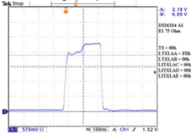
E1 75 Min Overshoot (1) Max (1CE)
