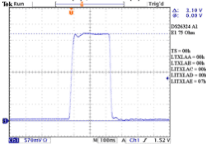
E1 75 Max DAC No Overshoot (1) Plateau (2)
