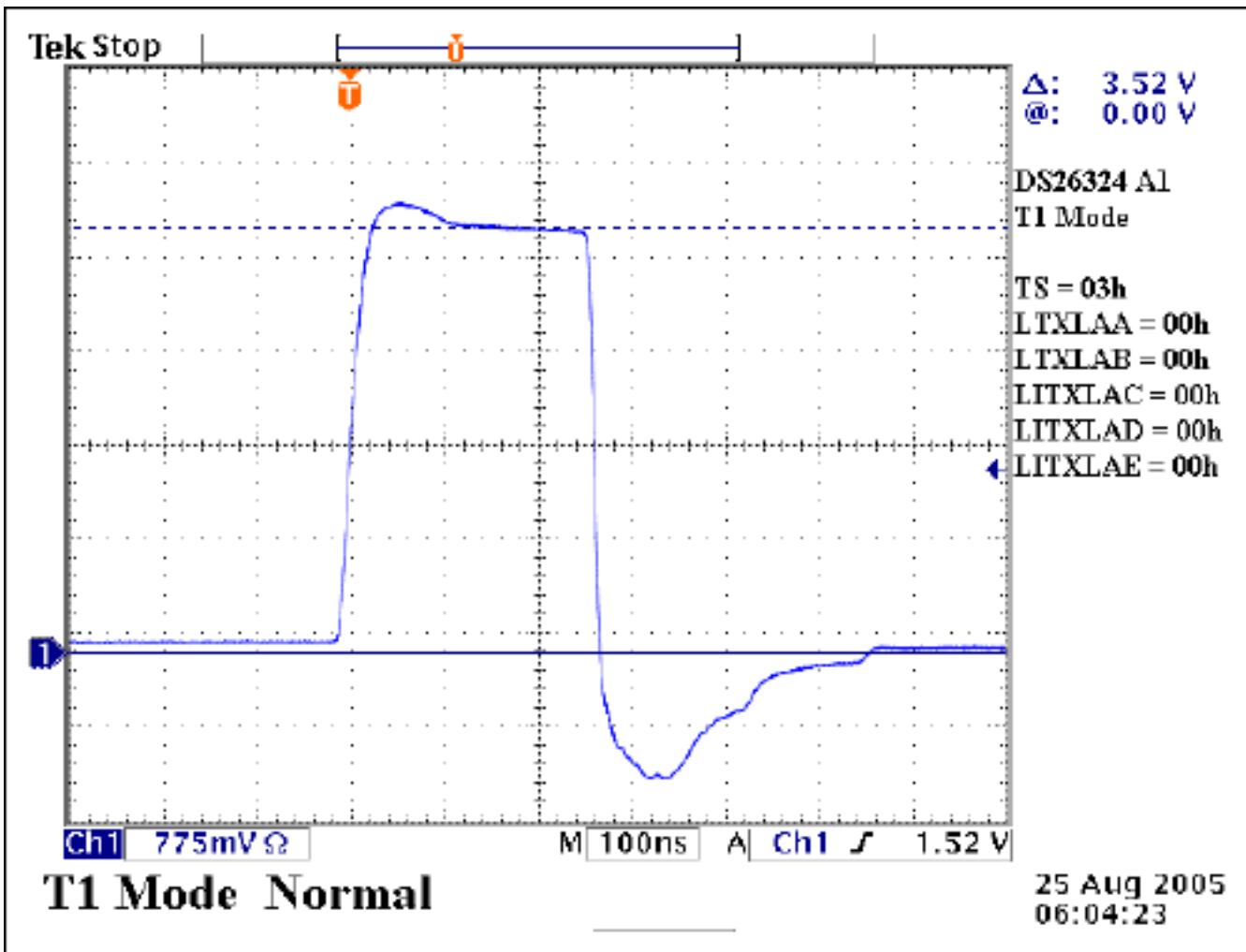
Figure 3. T1 normal operation.
