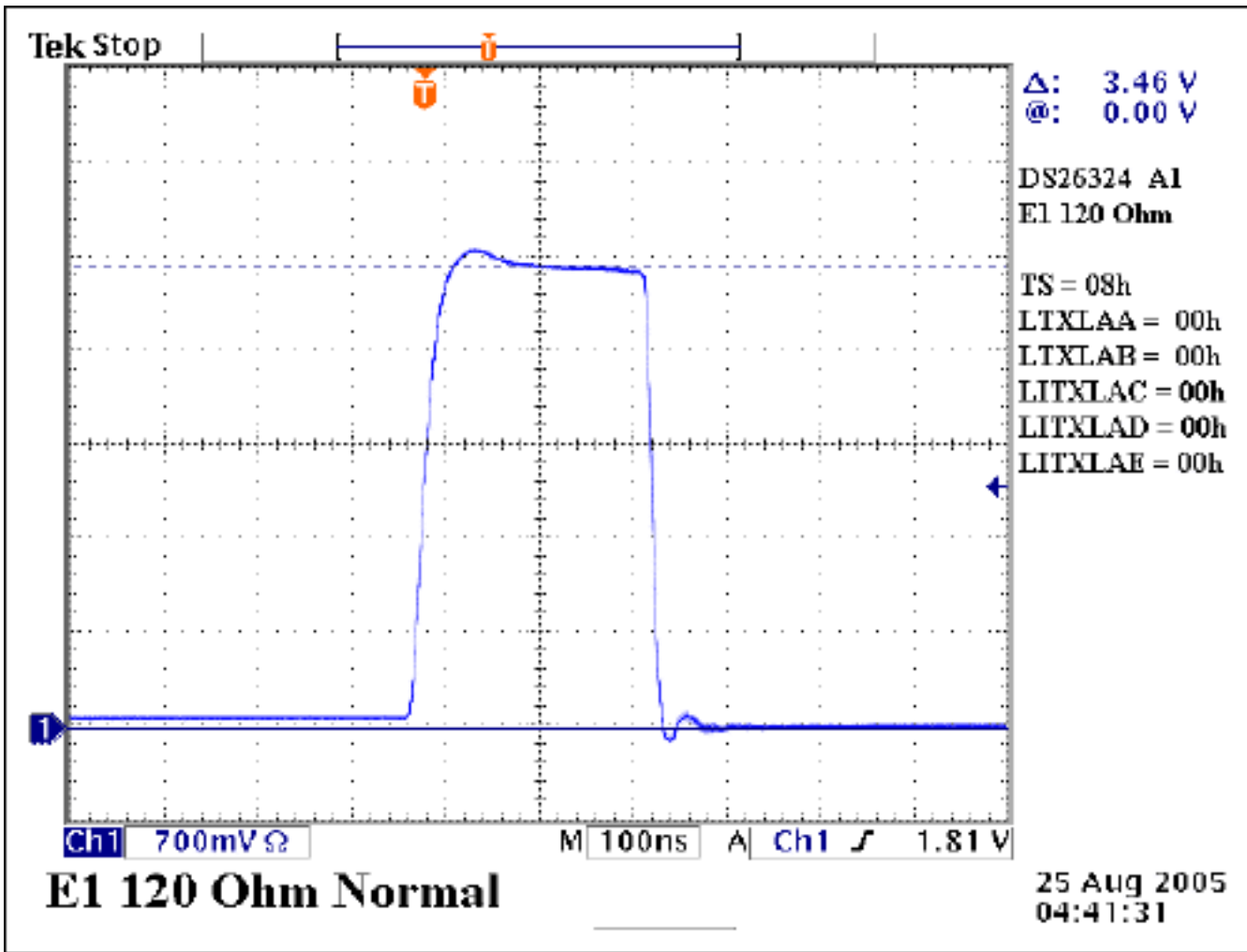
Figure 4. E1 120Ω normal operation.
