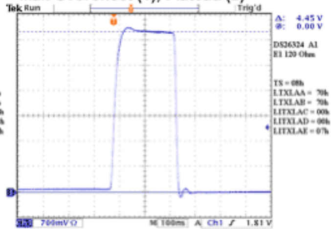
E1 120 Max DAC Max Overshoot (1) Plateau (2)
