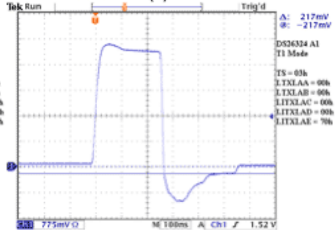
T1 Max Undershoot (5)
