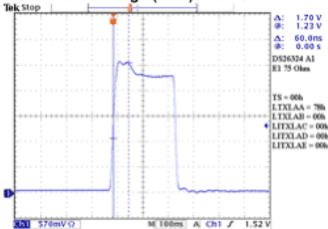
E1 75 Max Overshoot (1) Norm (1CE)
