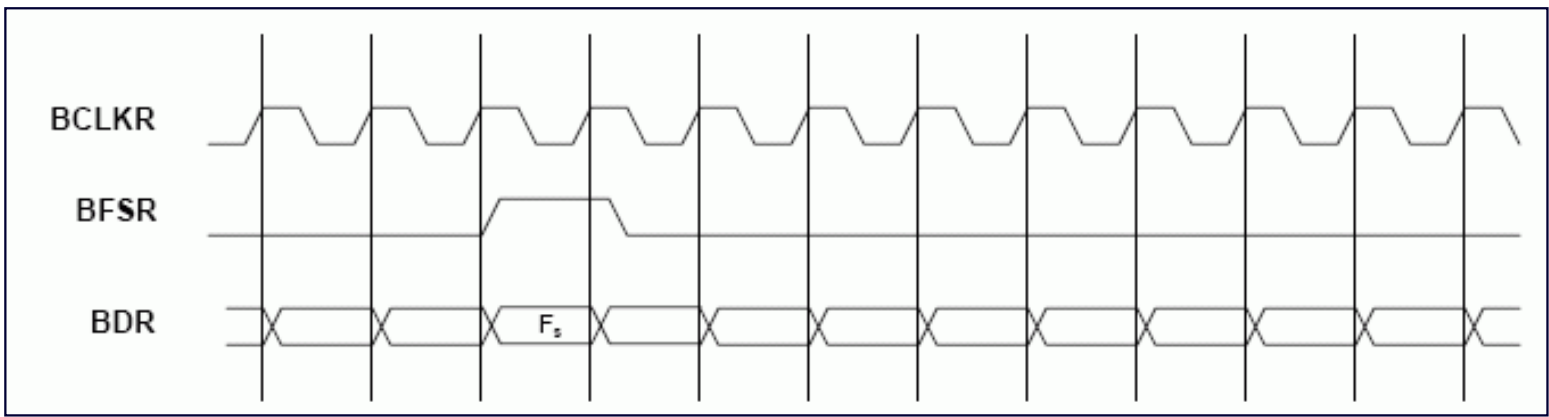
Figure 2. Continuous Mode Receive Timing (External Frame).
