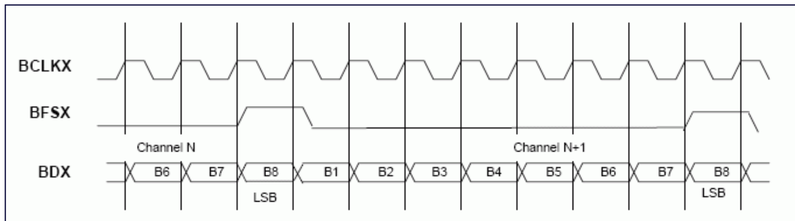
Figure 3. Burst Mode Transmit Timing (External Frame).
