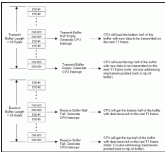
Figure 8. Autobuffering Unit Operation.
