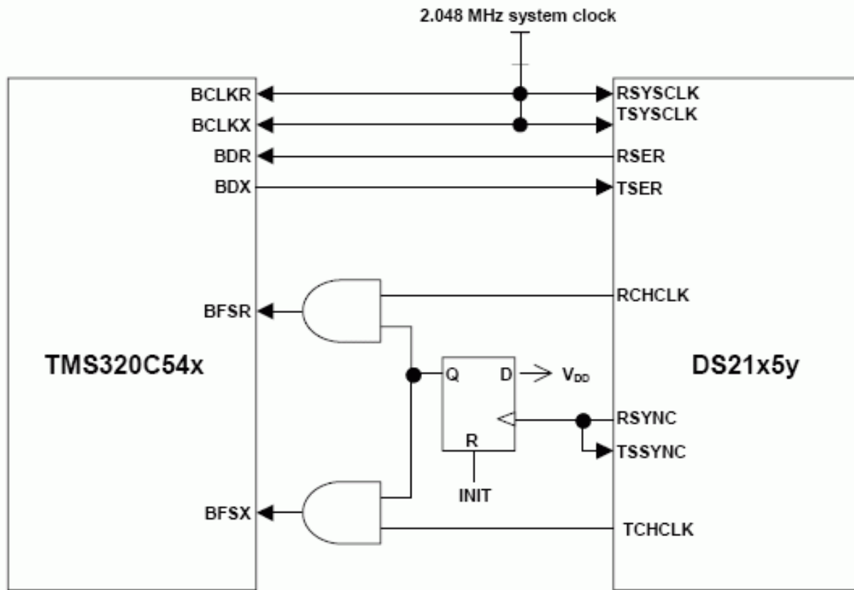
Figure 7. Block Diagram of the TMS320C54x and the DS21x5y Using a 2.048MHz System Clock Locked to the Network Clock.
