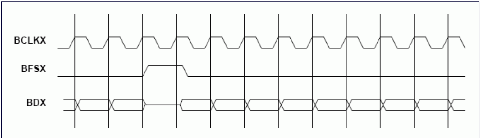
Figure 1. Continuous Mode Transmit Timing (External Frame).
