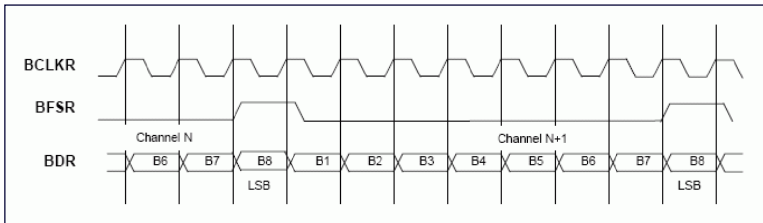
Figure 4. Burst Mode Receive Timing (External Frame).
