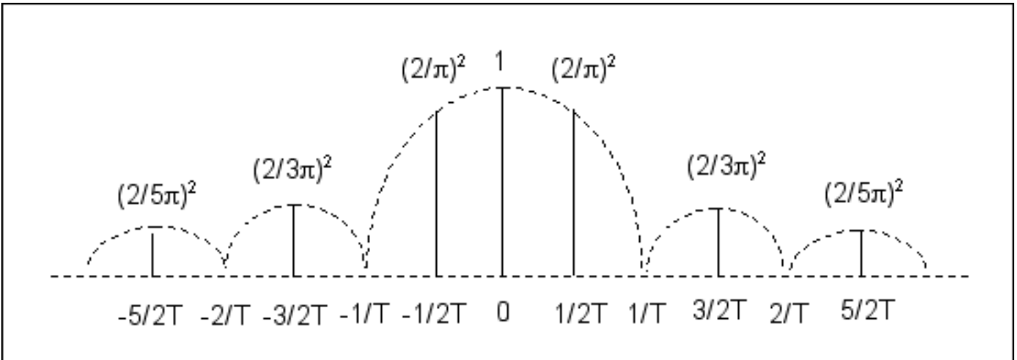
Figure 2. Power spectrum of a square wave of period 2T .
