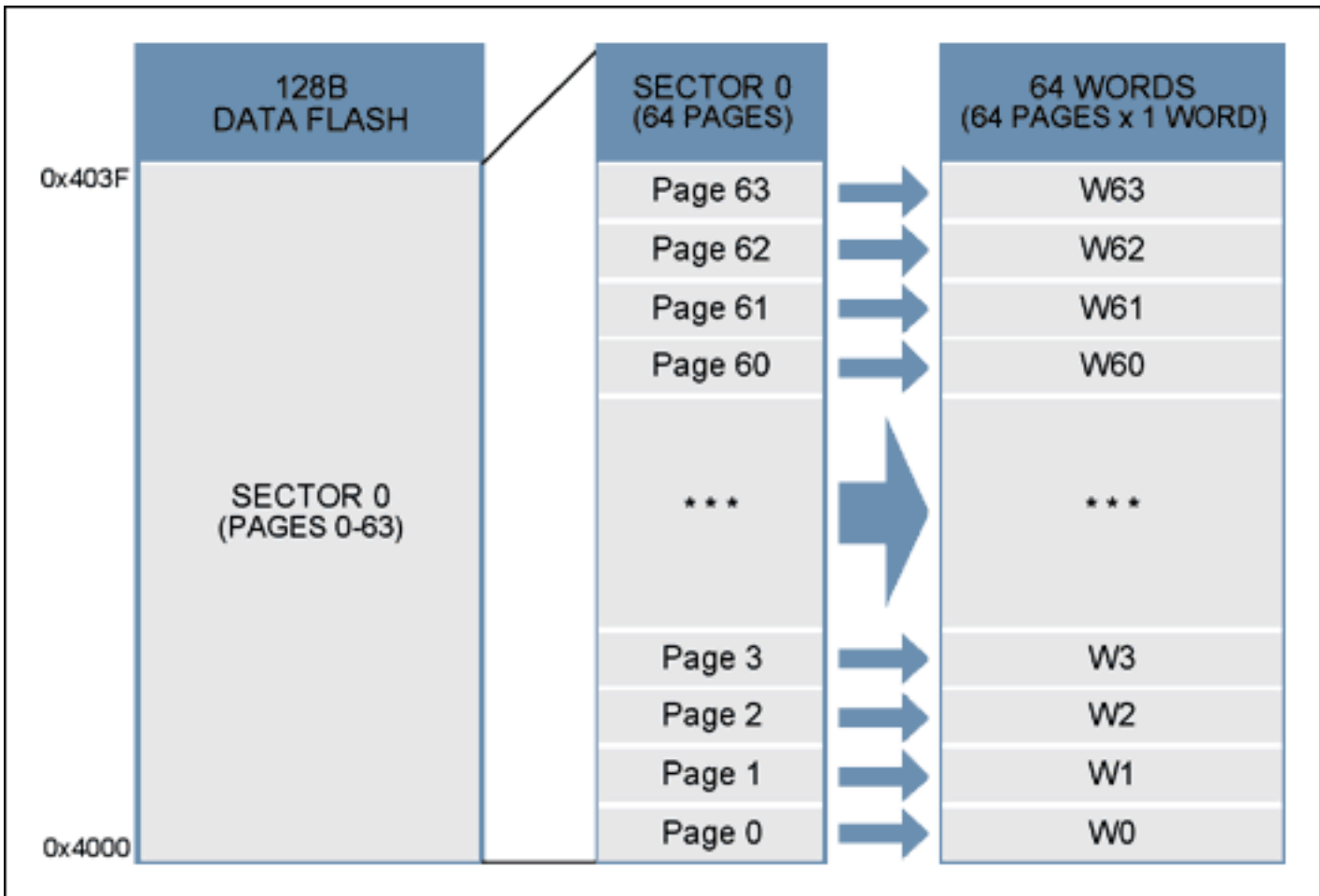
Figure 2. Sector/page structure for 128B data flash.
