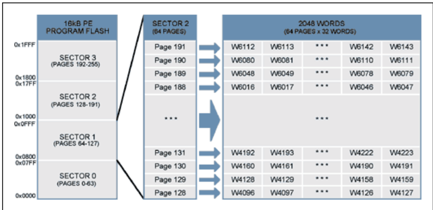
Figure 1. Sector/page structure for 16KB program flash.
