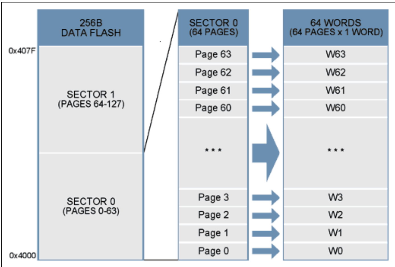
Figure 2. Sector/page structure for 256B data flash.
