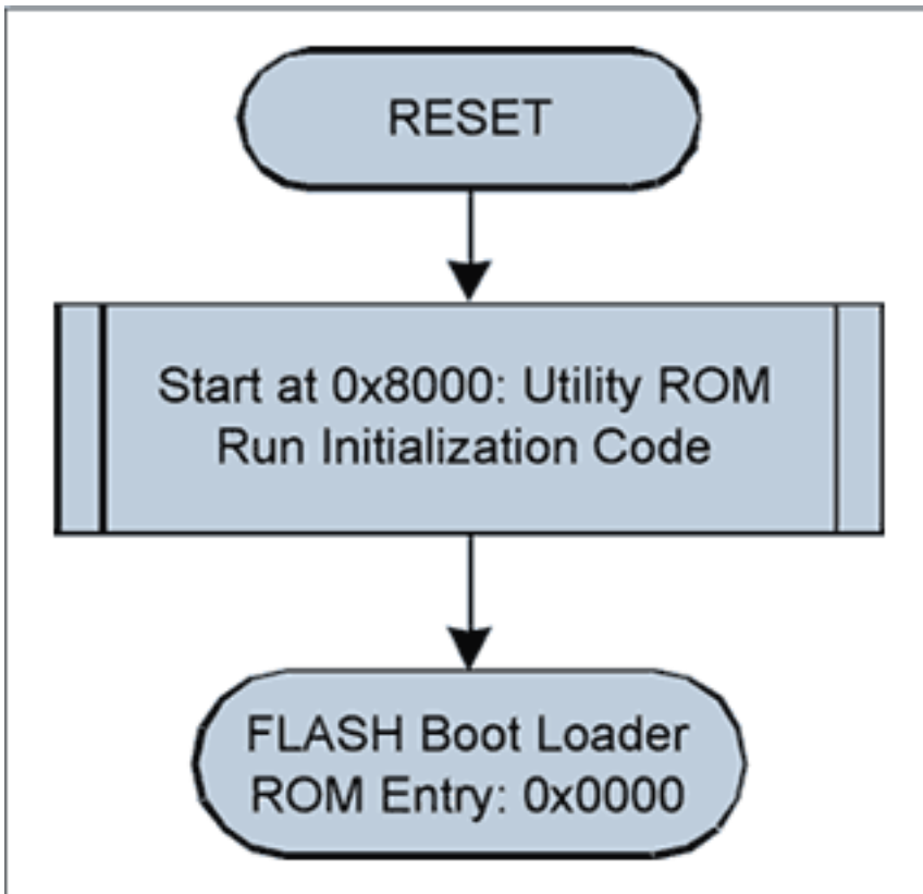
Figure 4. Flowchart of a simplified ROM initialization.
