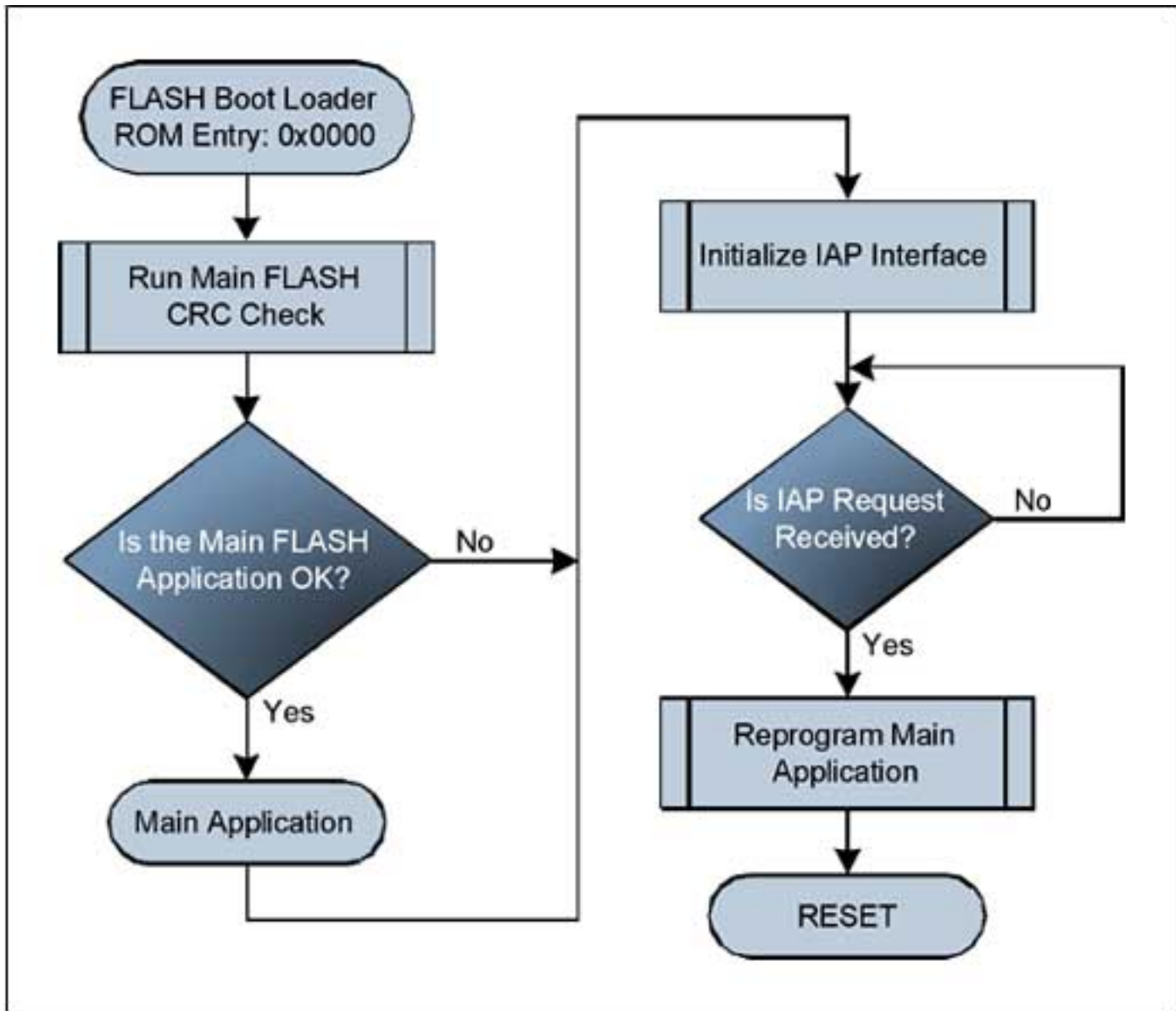
Figure 5. Flowchart for a simplified flash boot loader.
