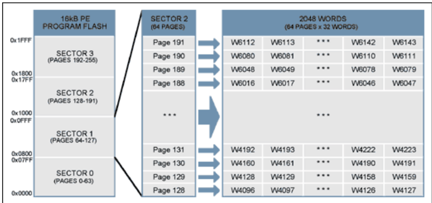
Figure 1. Sector/page structure for 16KB program flash.
