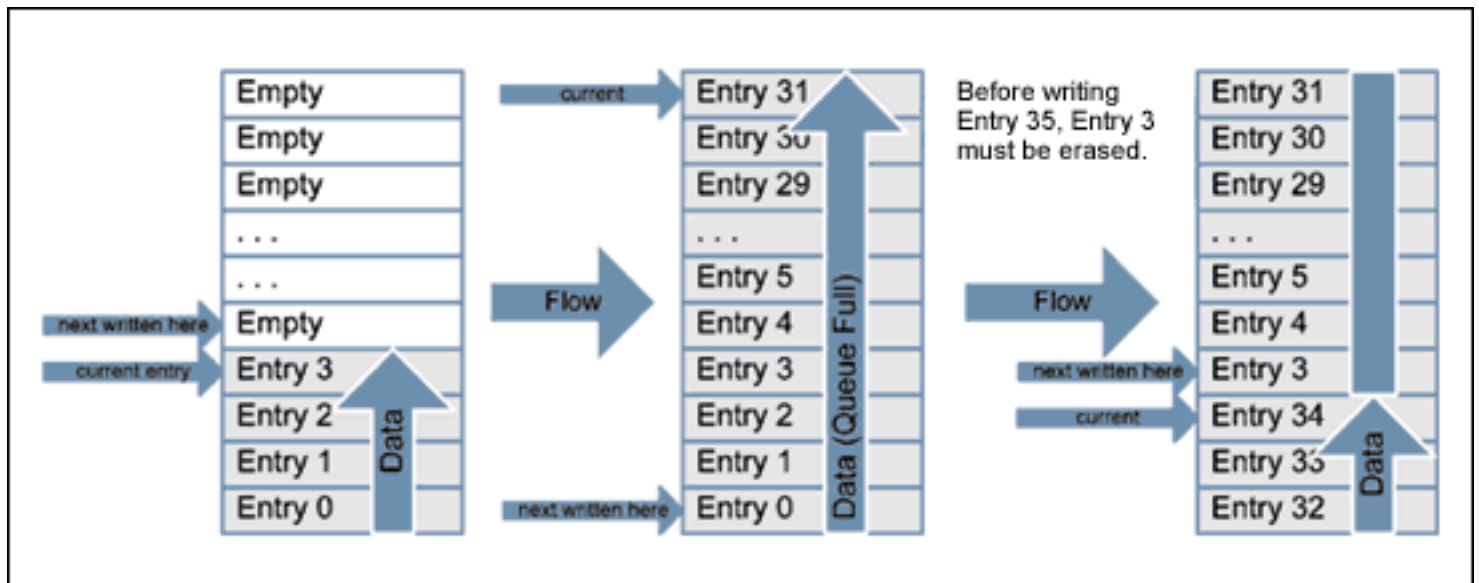
Figure 3. Diagram of a bounded queue flow.
