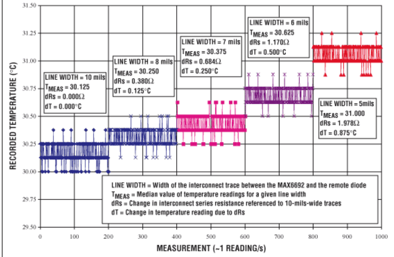
Figure 1. The effect of DXN-DXP line width on temperature measurement is shown. Smaller line widths have higher series resistance and, therefore, increase the measured temperature by 0.45^\circ\text{C}/\Omega .
