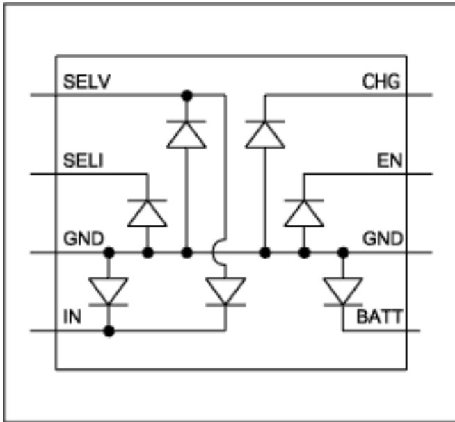
Figure 2. MAX1811 on-chip ESD diodes allow direct measurement of junction temperature.
