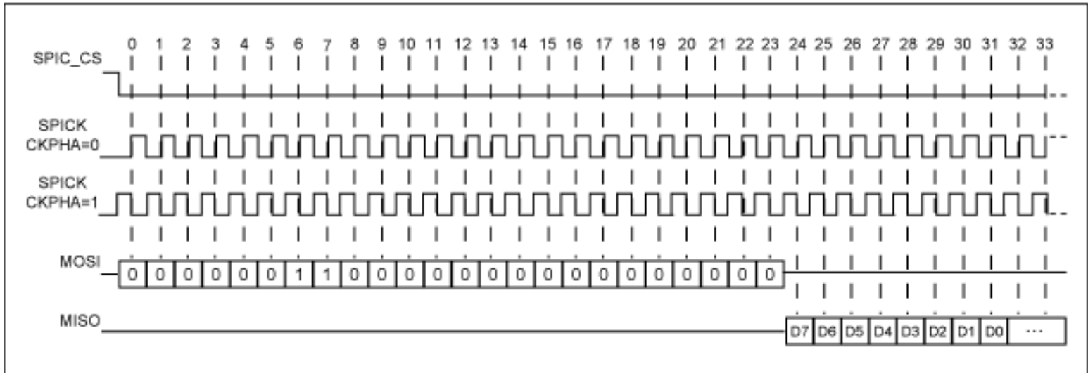
Figure 1. SPI master functional timing.
