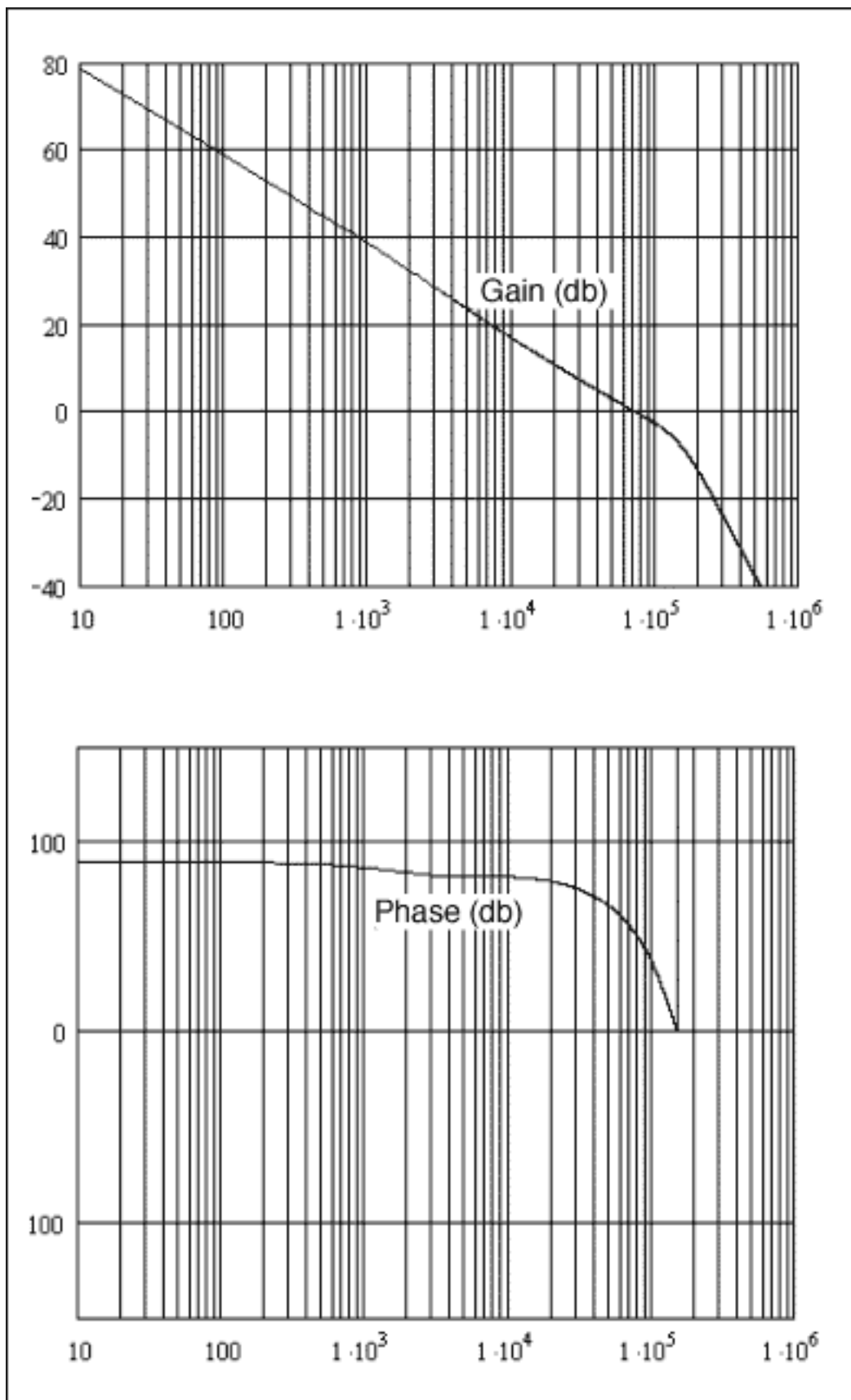
Figure 4. Open-loop gain and phase plots from MathCad.
