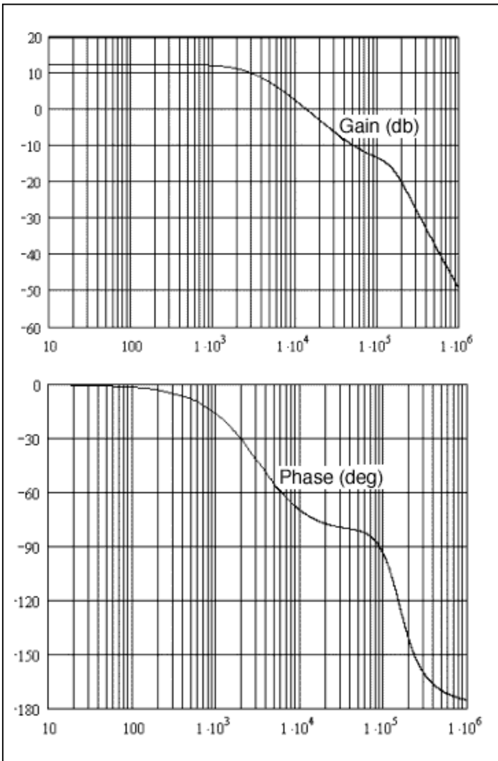
Figure 3. Control-to-output gain and phase plots from MathCad.
