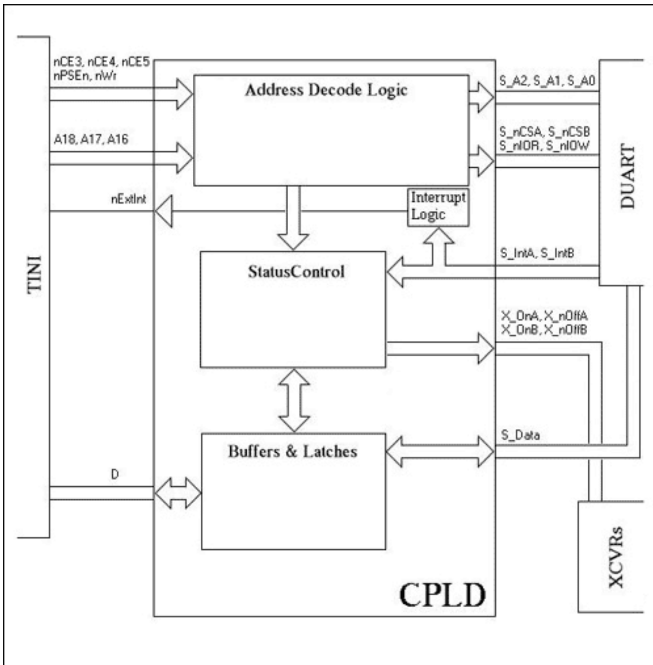
Figure 2. CPLD interface.
