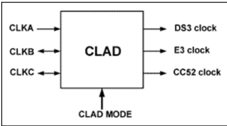
Figure 1. CLAD block for the DS318x.
