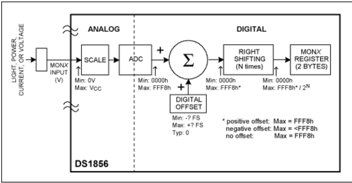
Figure 1. DS1856 MON input block diagram.
