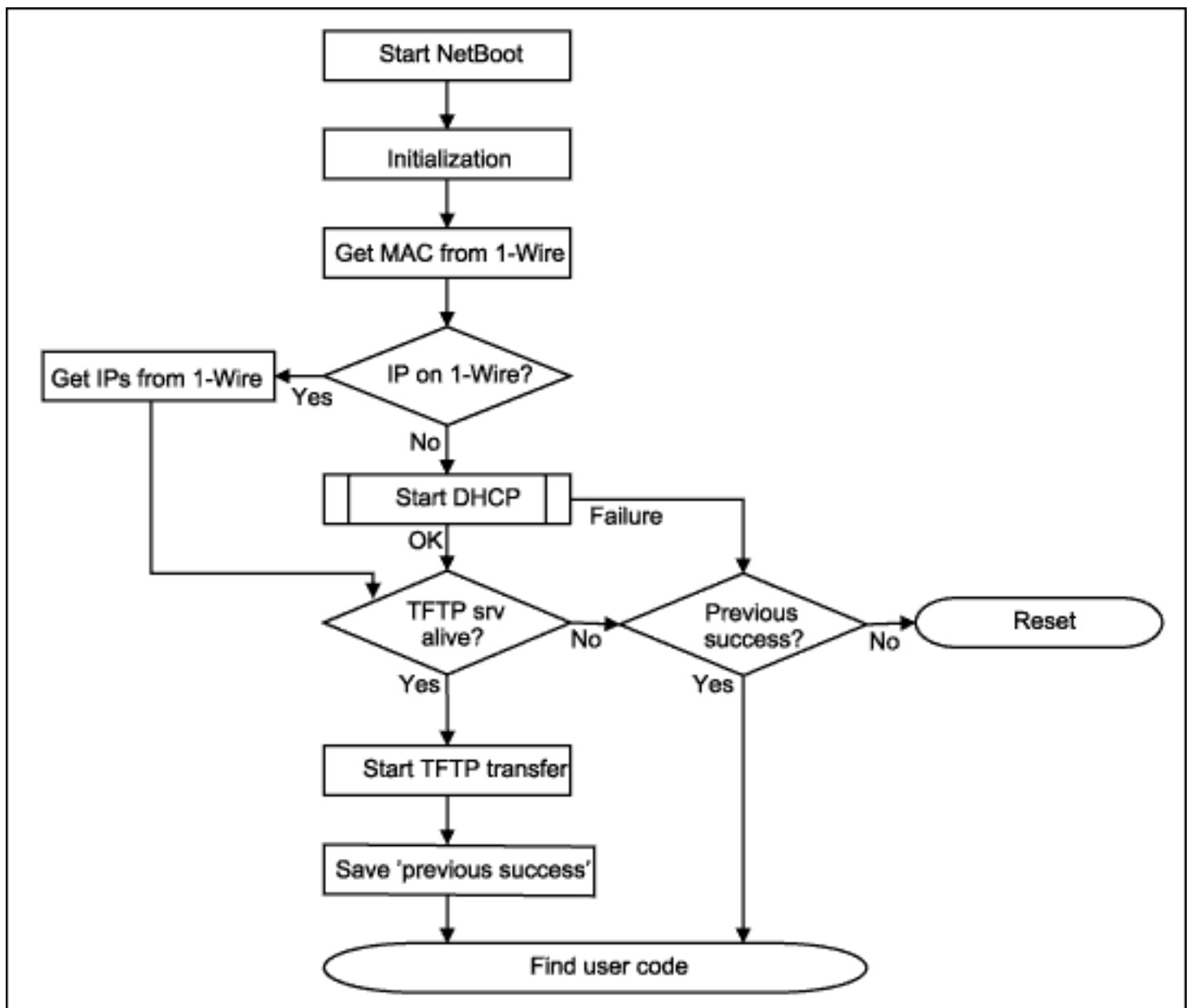
Figure 1. NetBoot process flowchart.
