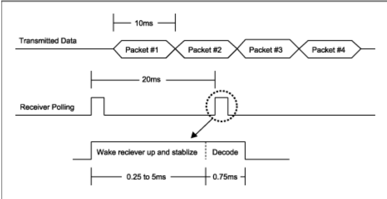
Figure 2. To monitor keyfob transmissions, an RKE receiver must allocate time to wake up and stabilize before decoding the incoming signal.
