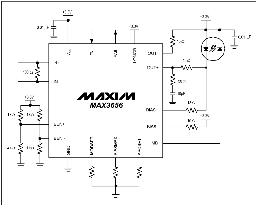
Figure 1. Application Circuit for the MAX3656
