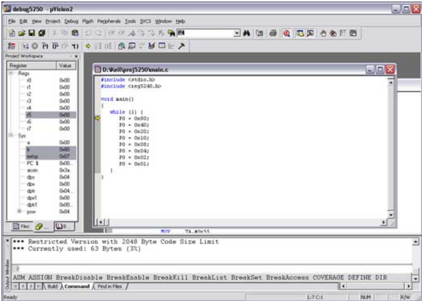
Figure 6. Debugging output from Keil μVision.
