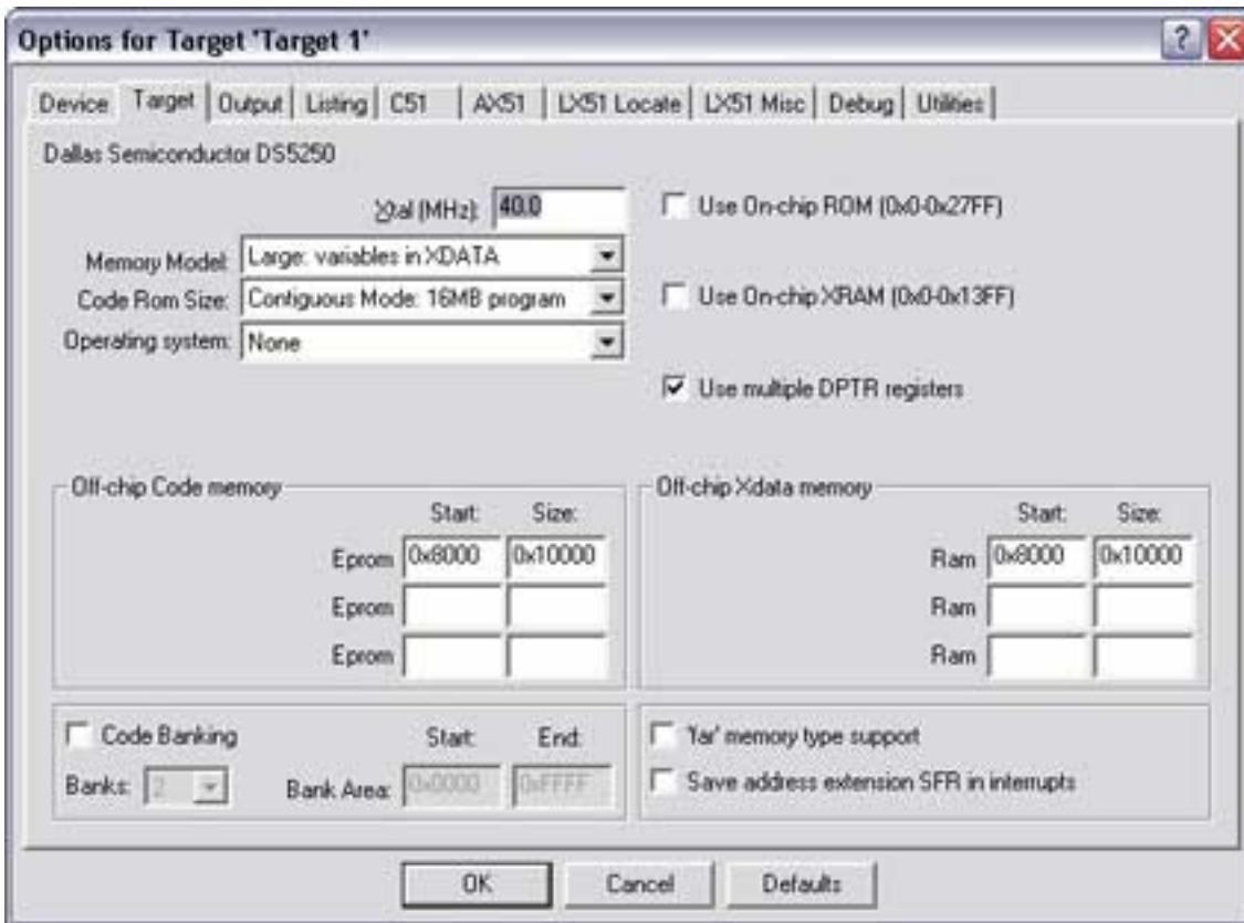
Figure 3. Target option settings for the DS5250.
