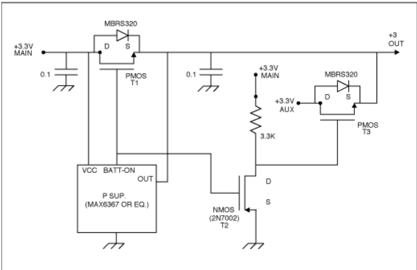
Figure 1. Power backup switch.
