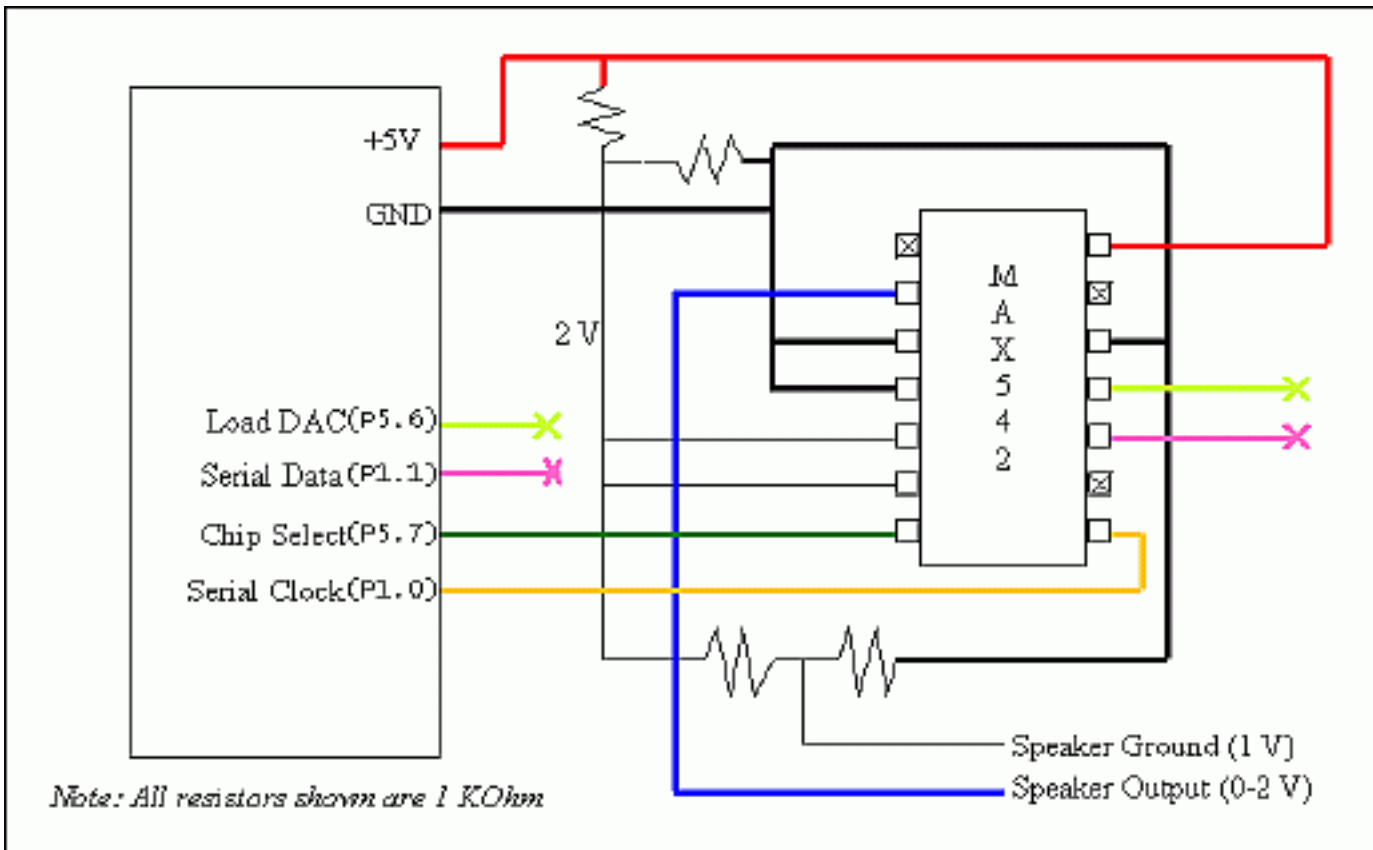
Figure 1. Hardware block diagram.
