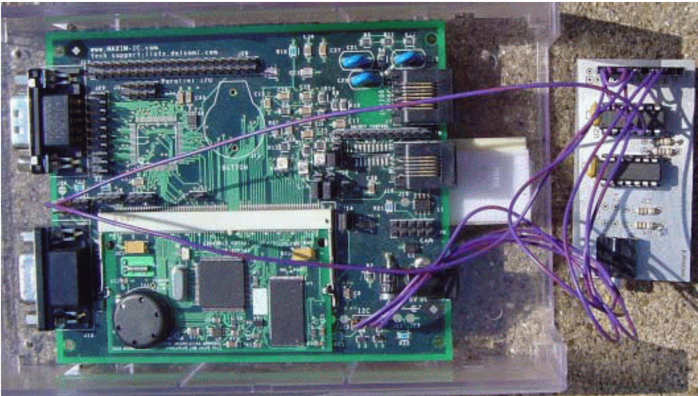
Figure 2. TINI connected to MAX542 DACs.
