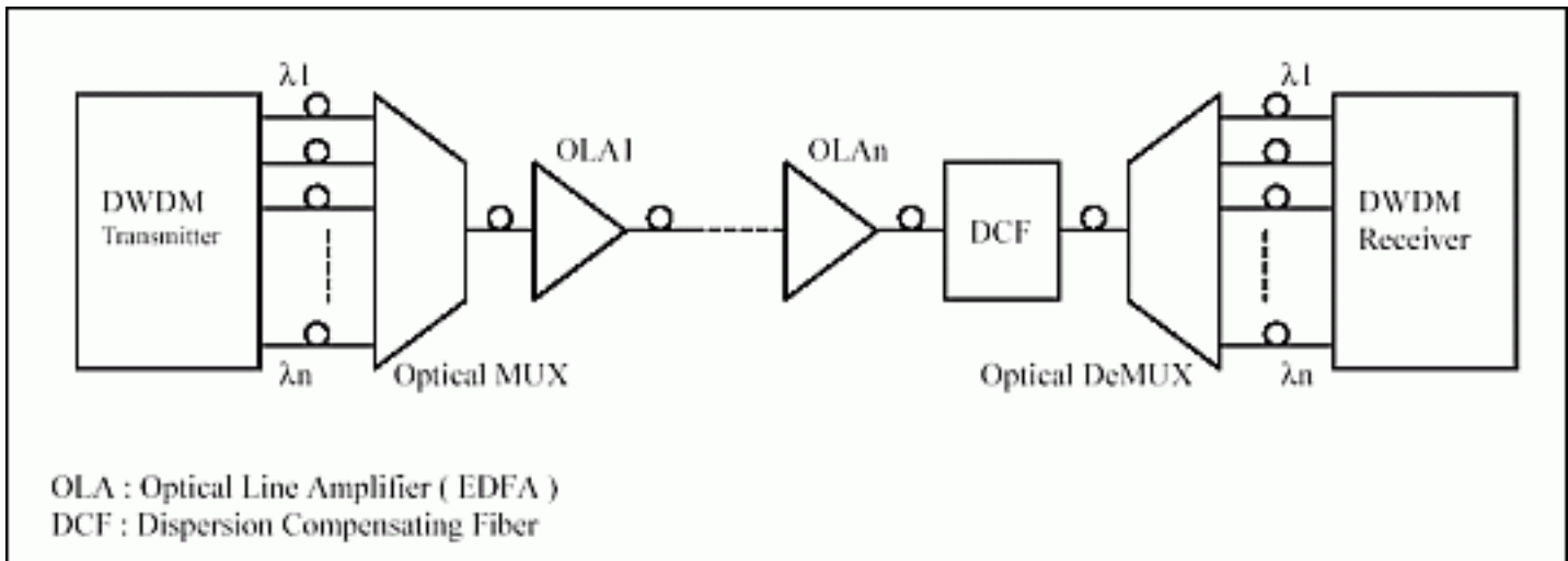
Figure 1. Example of a dense wavelength-division multiplex (DWDM) link.
