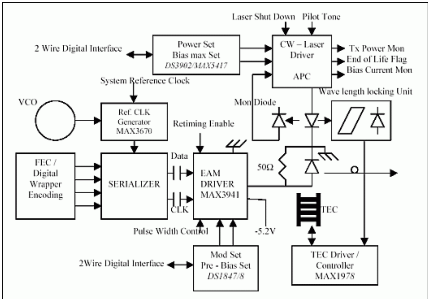
Figure 2. Example of a 10Gbps DWDM transmitter.
