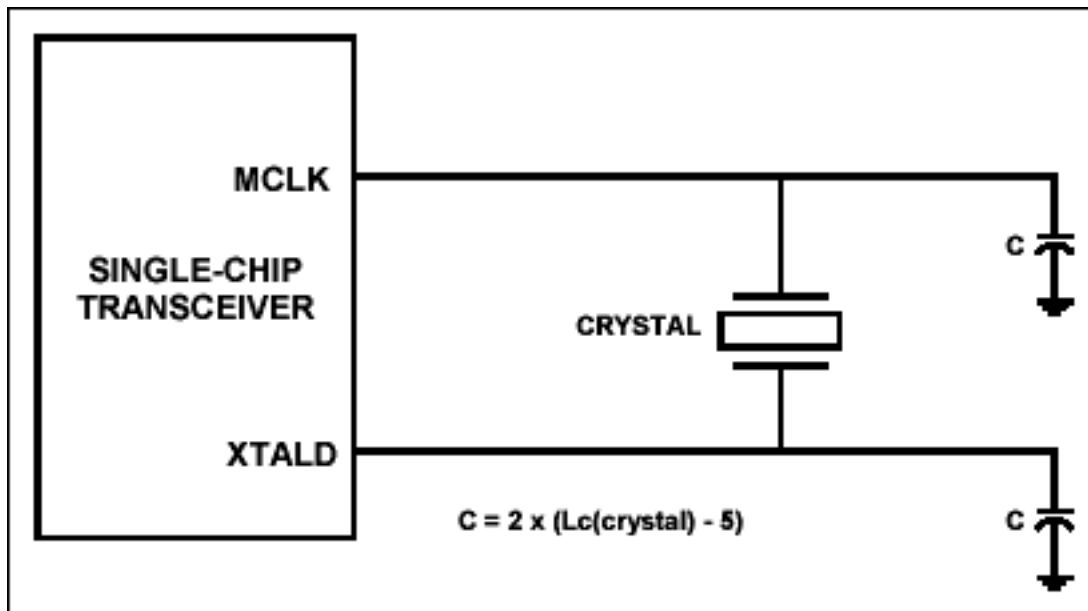
Figure 1. Crystal connection.
