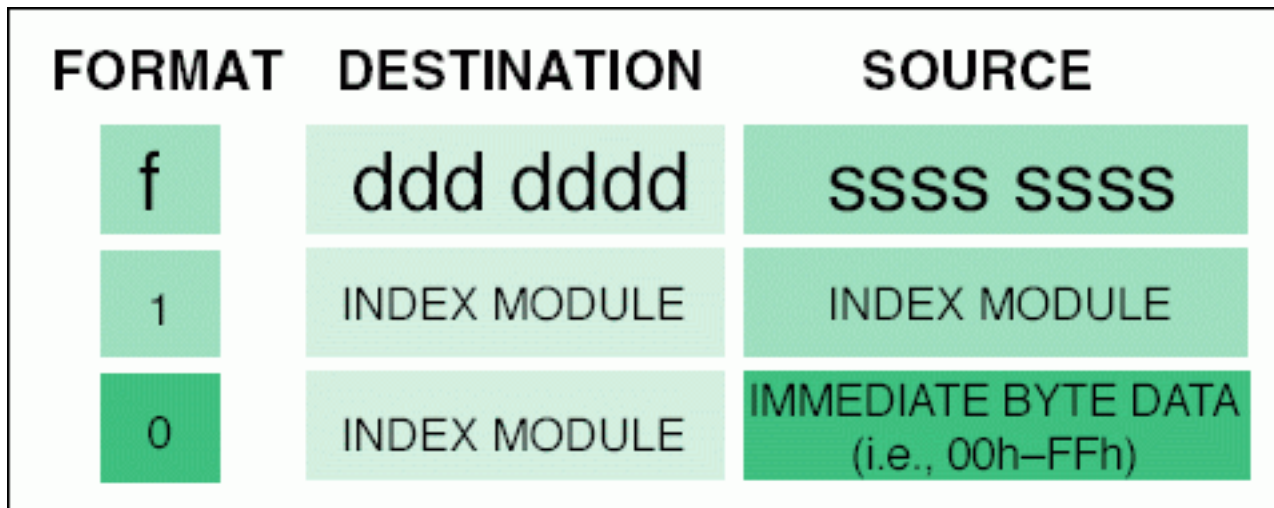
Figure 1. The MAXQ instruction word is simple, yet very powerful.
