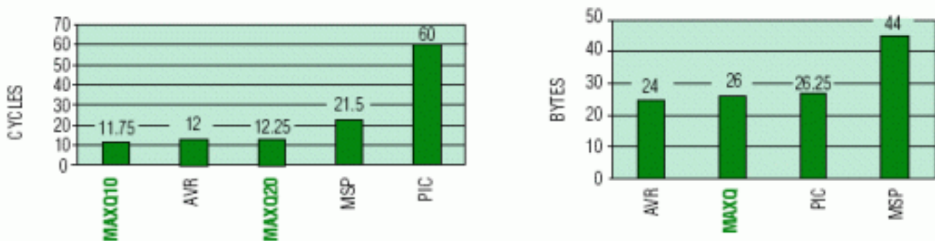
Hex2Asc CYCLE/BYTE COUNT COMPARISON
