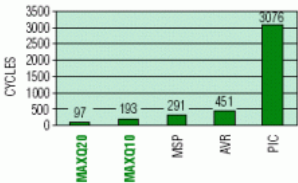
MemCpy64 CYCLE/BYTE COUNT COMPARISON
