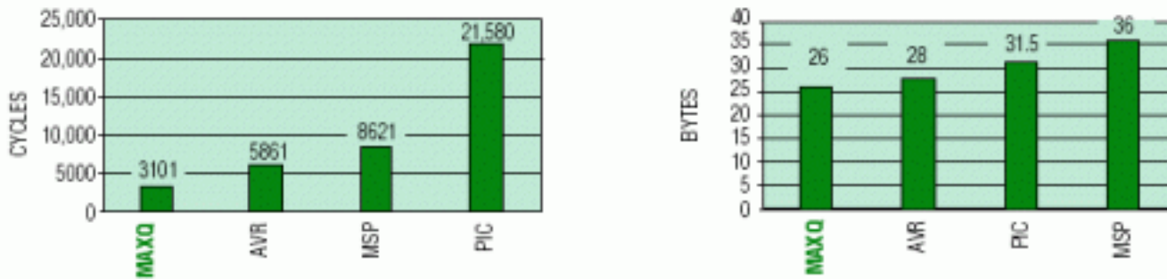
BubbleSort CYCLE/BYTE COUNT COMPARISON
