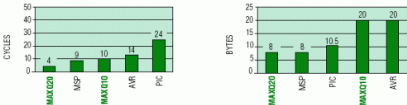
ShRight CYCLE/BYTE COUNT COMPARISON
