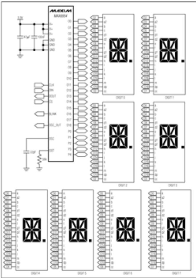
Figure 1. MAX6954 16-segment application circuit.
