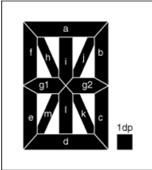
Figure 2. Segment labeling for 14-segment displays.
