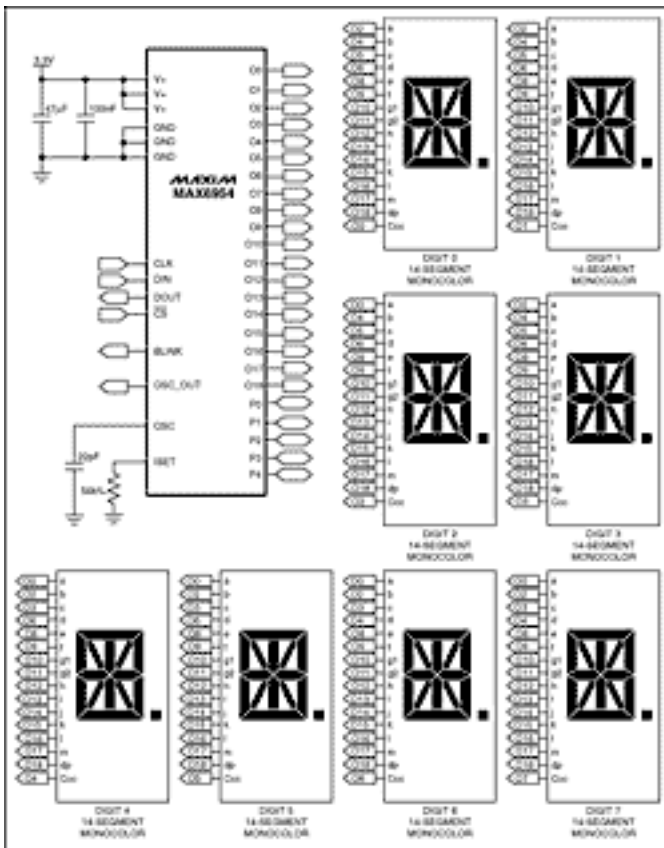
Figure 1. MAX6954 14-segment application circuit.
