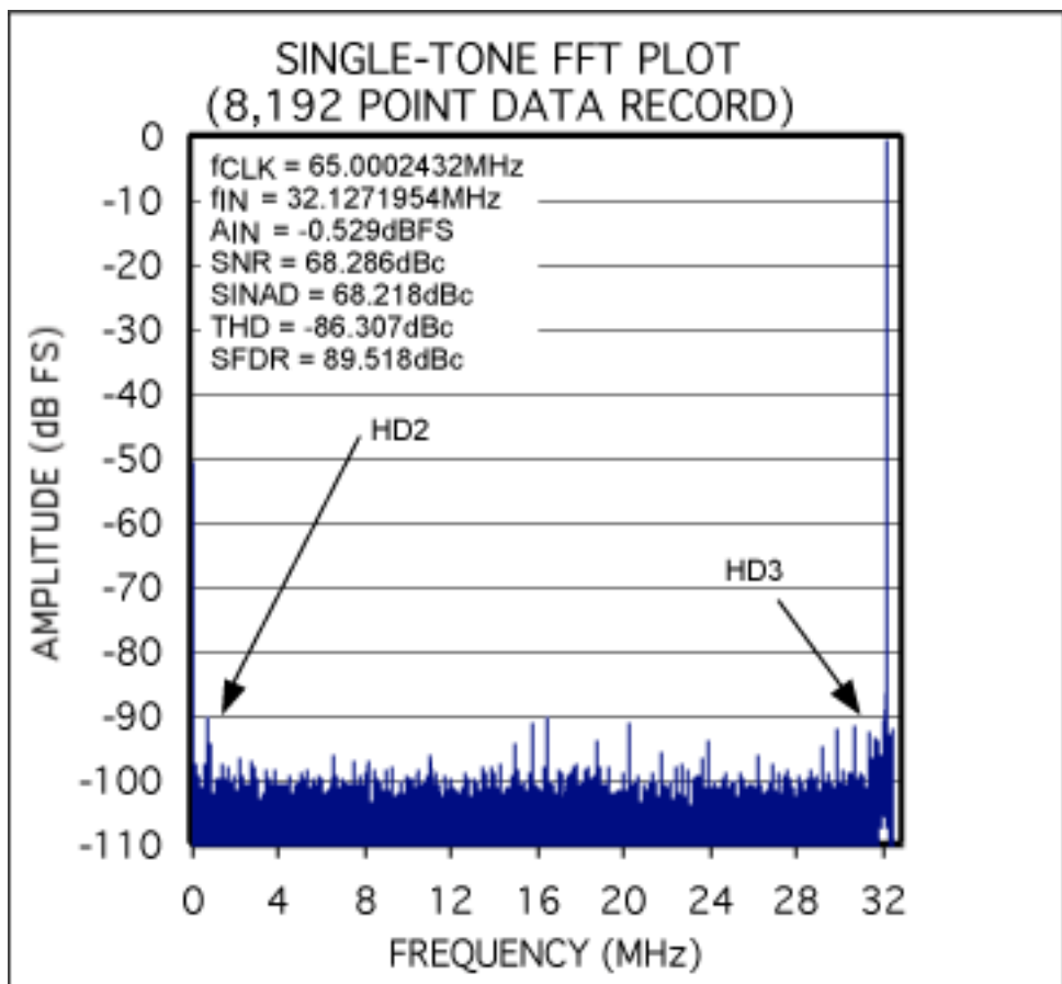
Figure 3. Coherently sampled FFT from the MAX1211EVKIT. f_{CIN}=32.1271954\text{MHz}
