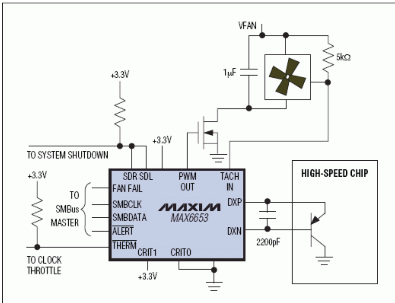
Figure 2. PWM-output temperature sensor and automatic fan-speed controller. Fan speed is controlled automatically based on temperature. Clock throttle and system shutdown outputs prevent a high-speed chip from reaching destructive temperatures. CRIT0 and CRIT1 pins can be strapped to supply or ground to select default shutdown-temperature thresholds, ensuring protection even when system software hangs.
